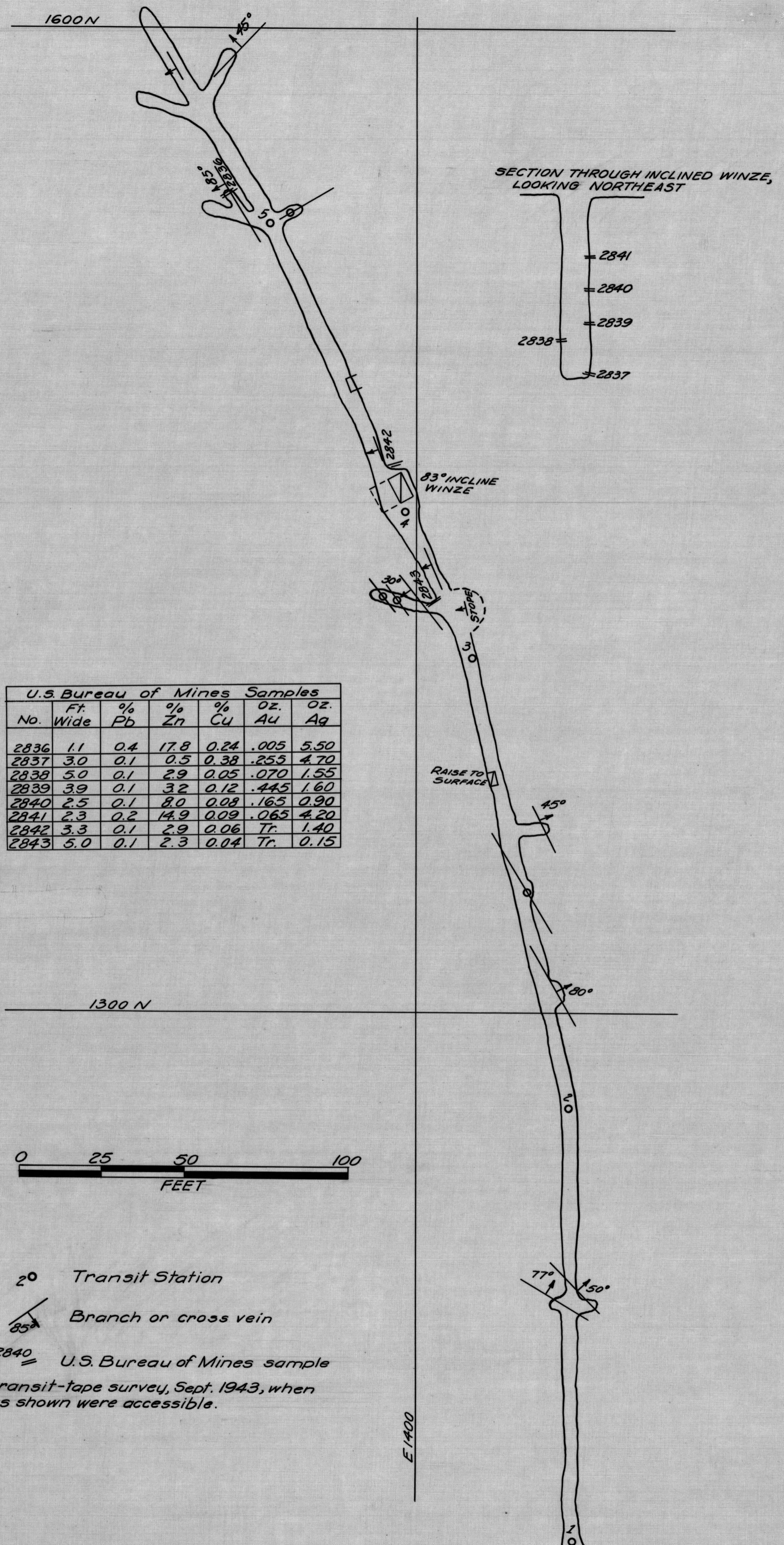
FIG. 15-PLAN OF UNDERGROUND WORKINGS, COLUMBUS MINE, MOHAVE CO., ARIZ.
