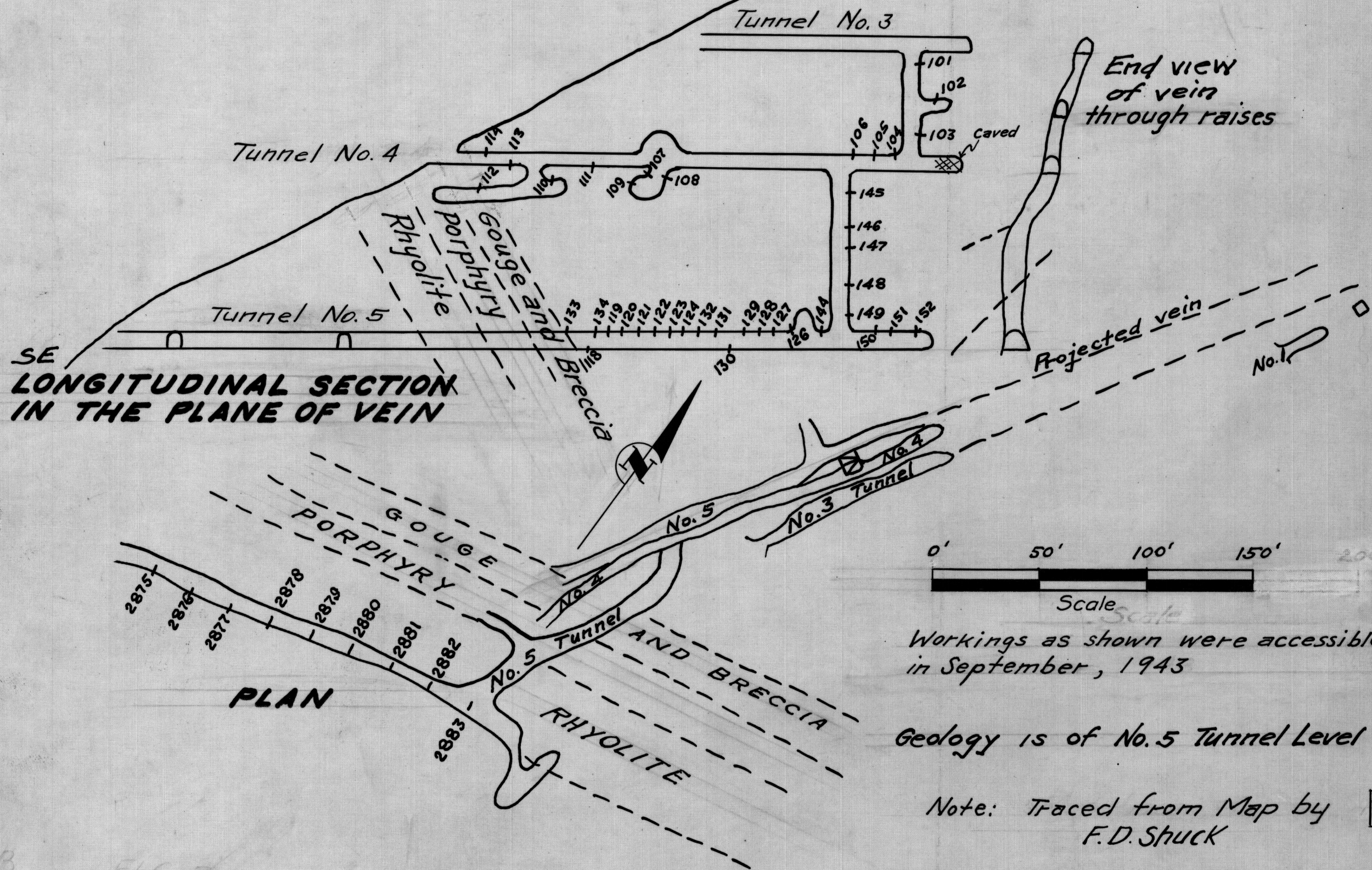
Fig. 3-Longitudinal Section in plane of vein, and Plan, EUREKA MINE, Mohave Co., Ariz
