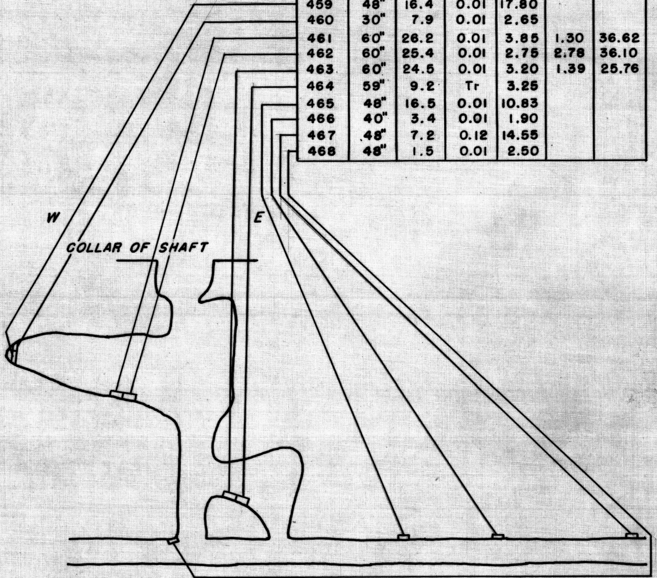
SECTION A-A' RATTLESNAKE SHAFT
