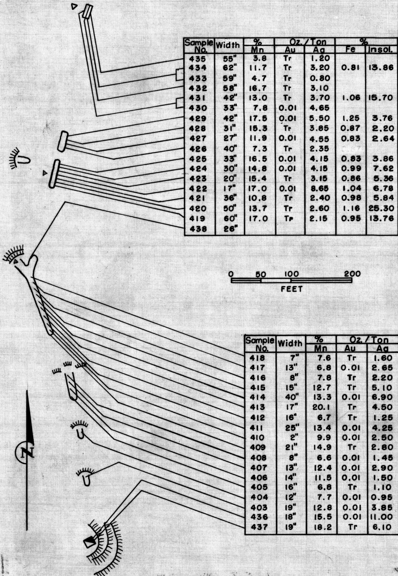
FIGURE 24. - ASSAY MAP OF BLACKTAIL CLAIM, SOUTH SECTION
