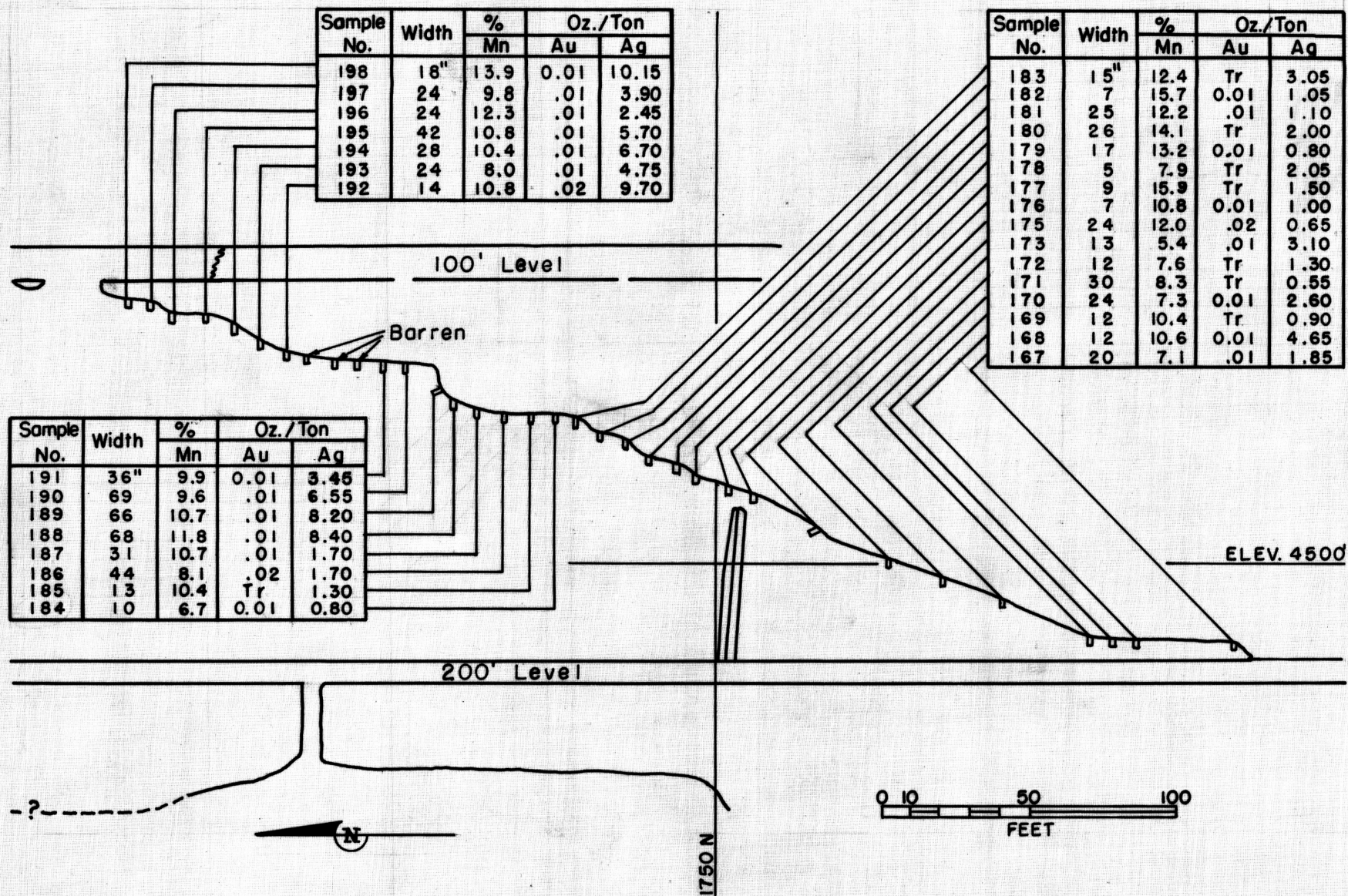
FIGURE 20. - SAMPLES BETWEEN COMET 200 LEVEL AND 100 LEVEL
