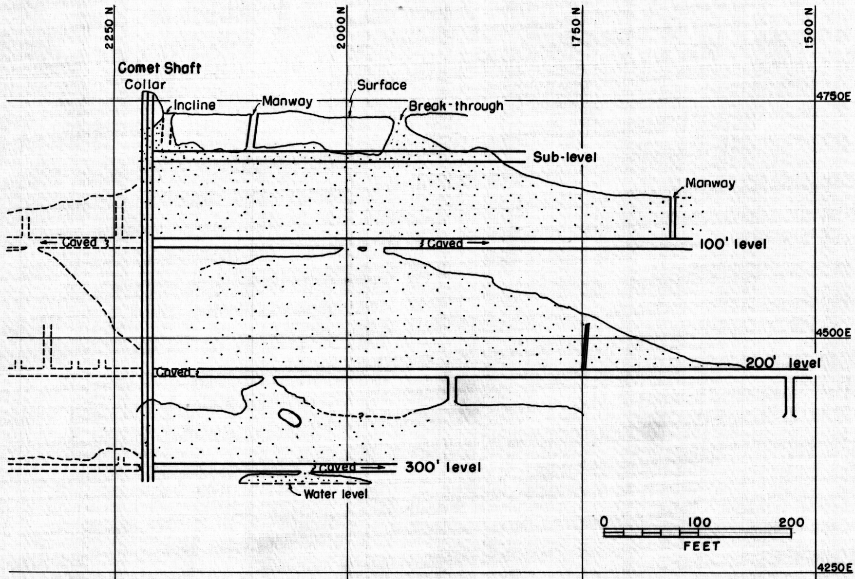
FIGURE 18. - LONGITUDINAL SECTION, SOUTH COMET AREA
