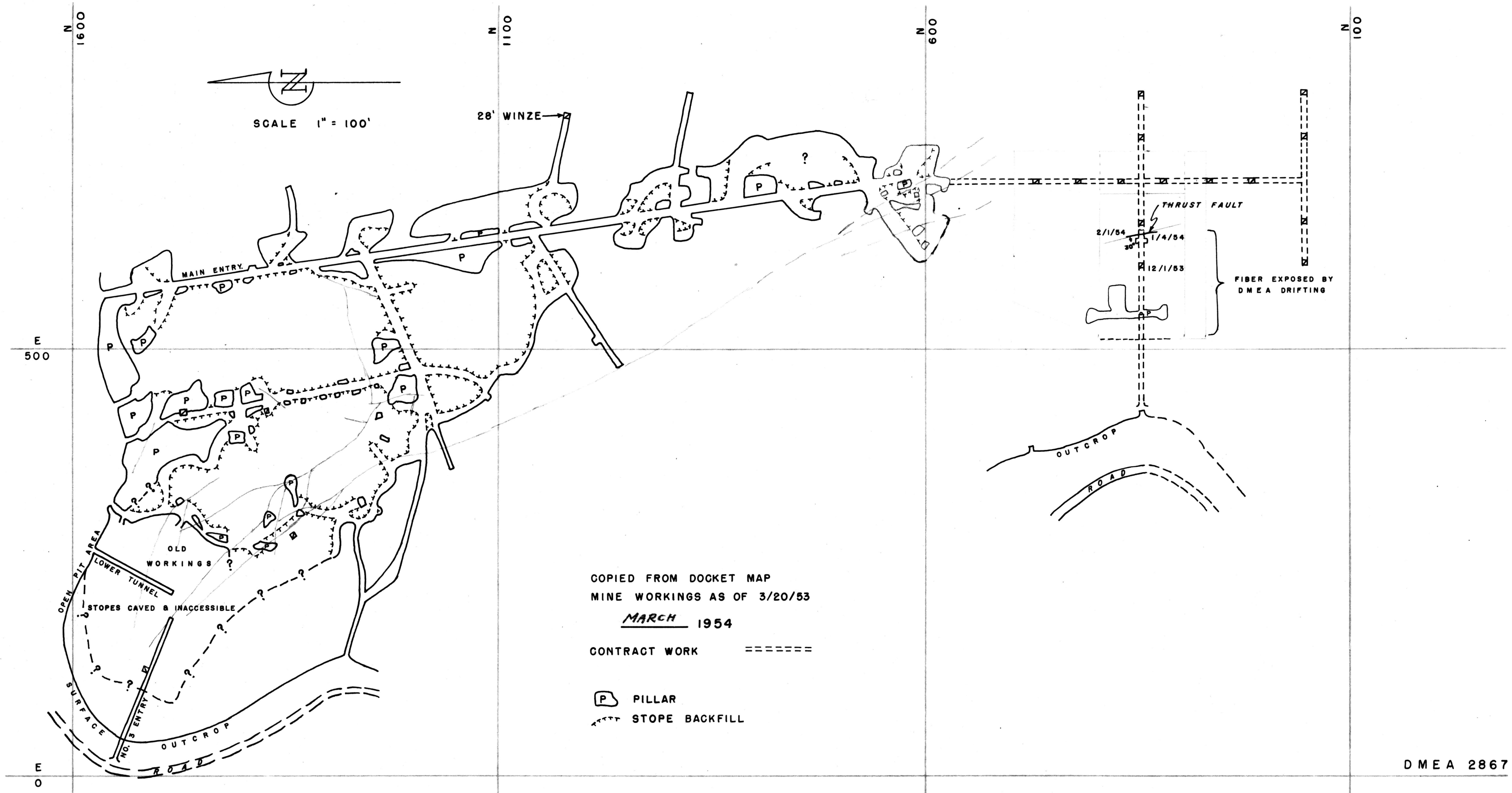
FIGURE 3. - MAP OF REGAL MINE, JAQUAYS MINING CORP., GILA COUNTY, ARIZONA
