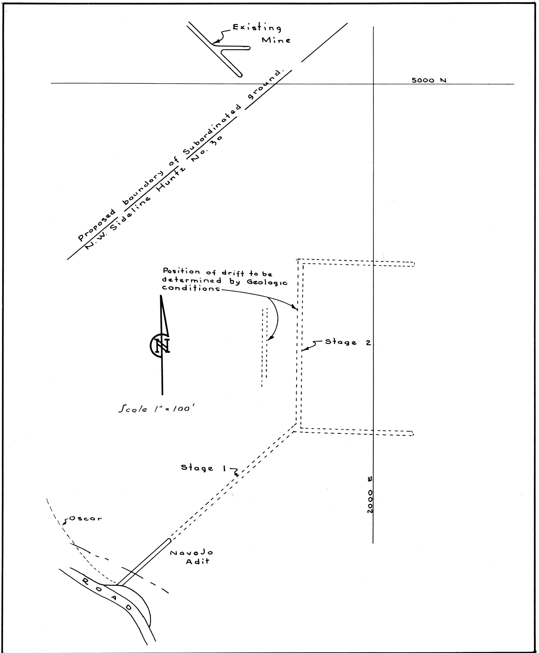
FIGURE - 4 - PROPOSED EXPLORATION SCHEME REGAL ASBESTOS MINE, GILA CO. ARIZONA
