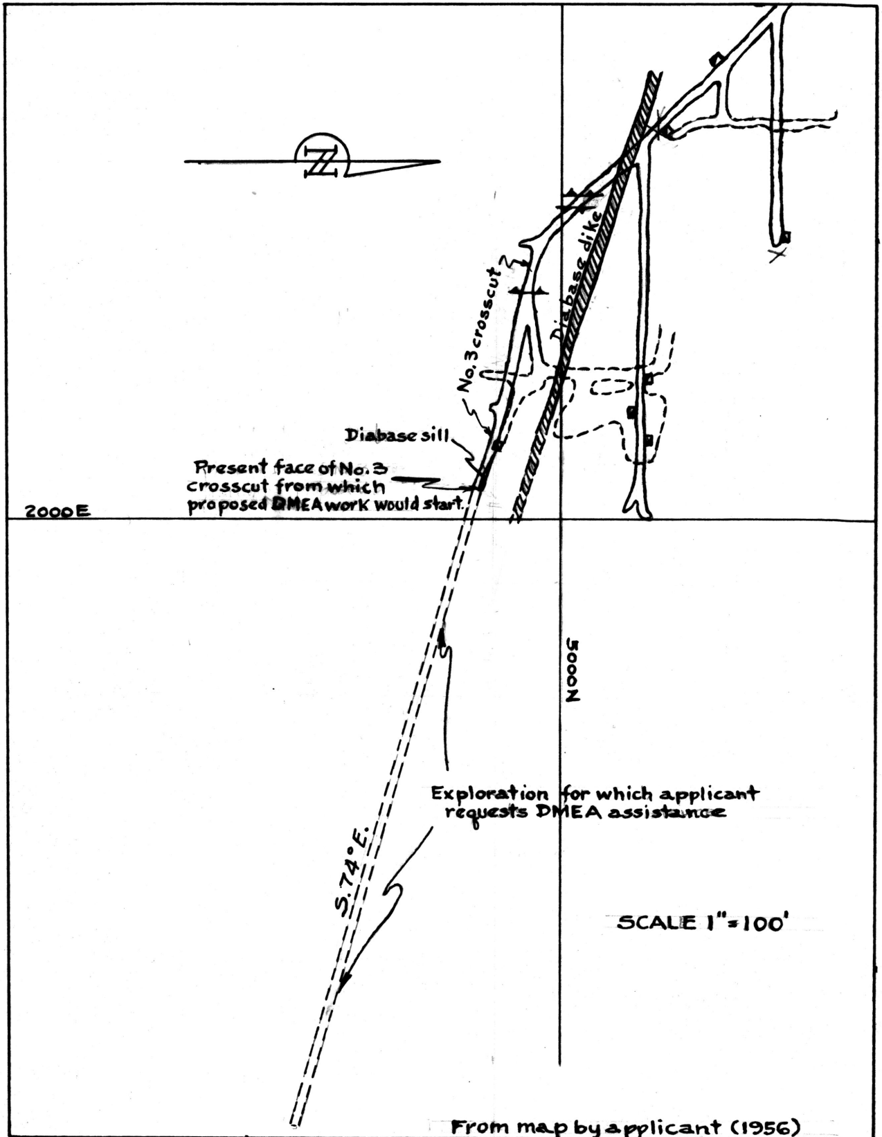
FIGURE 3A.- PLAN OF SOUTH WORKINGS OF REGAL MINE AND PROPOSED PROJECT (DMEA 3707).
