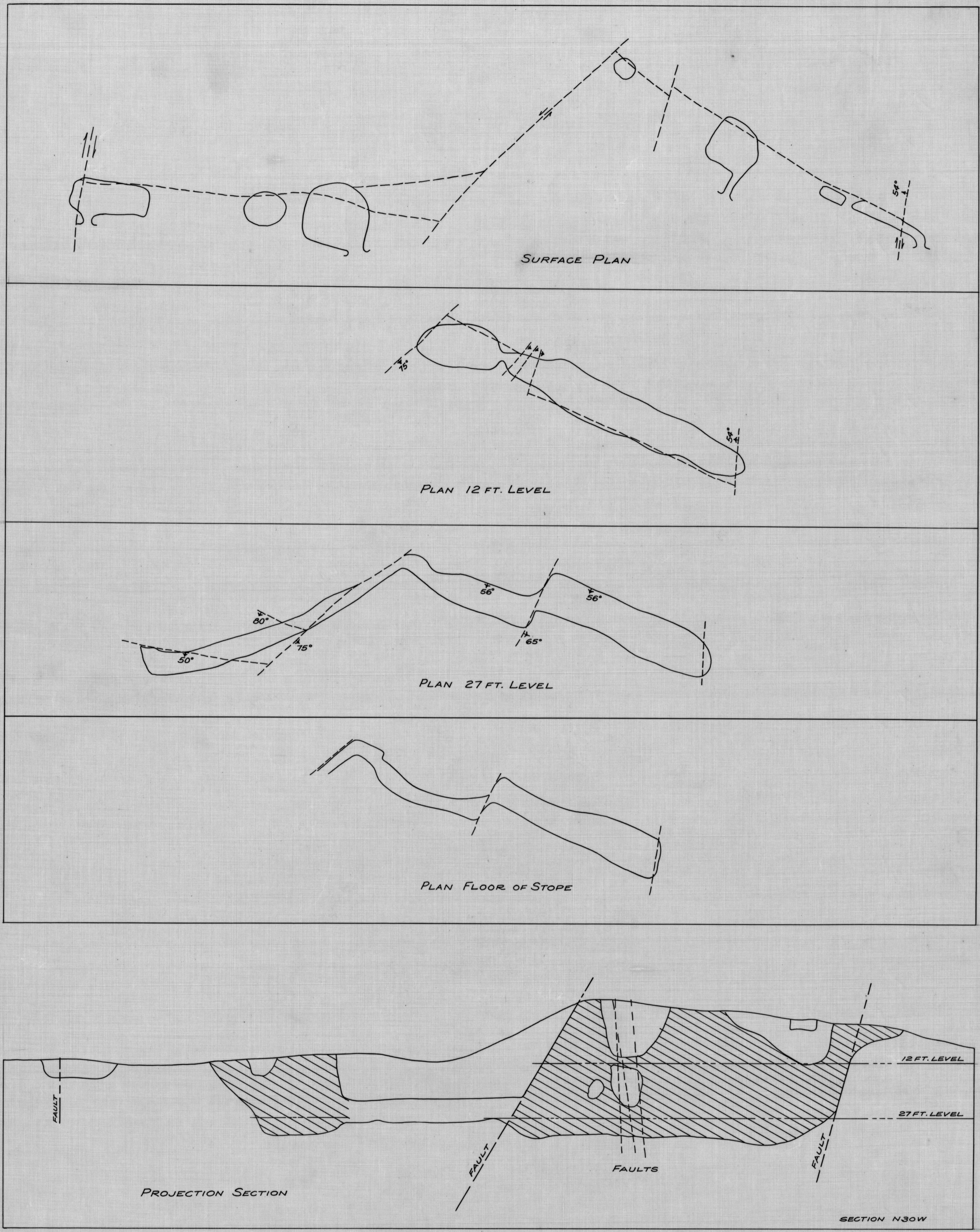
Fig. 4 BUREAU OF MINES FLOOR PLANS AND SECTION OF STOPE - BLACK QUEEN MINE AGUILA DISTRICT MARICOPA COUNTY, ARIZONA SCALE: 1 INCH = 20 FEET ENGINEER: G. A. APPELL DATE: 4-14-41 PREPARED BY: V. JOHNSON, U.S.G.S. TRACED BY: B. THOMPSON APPROVED BY: [Signature]
