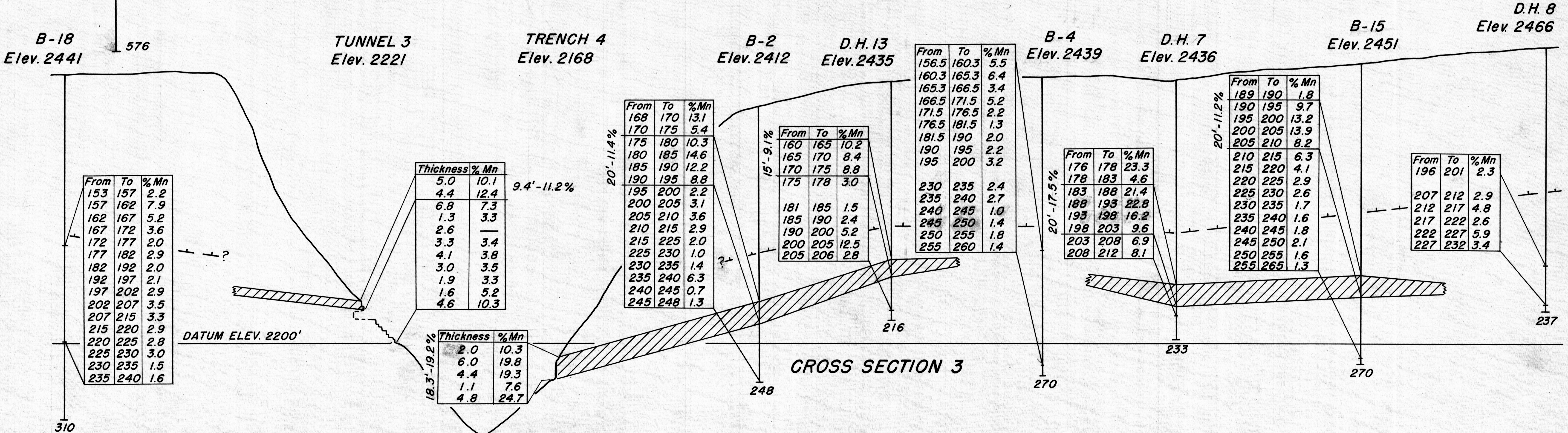
FIG. 7 - CROSS SECTIONS 3 & 8, ARTILLERY PEAK MANGANESE DEPOSIT, MOHAVE COUNTY, ARIZONA
