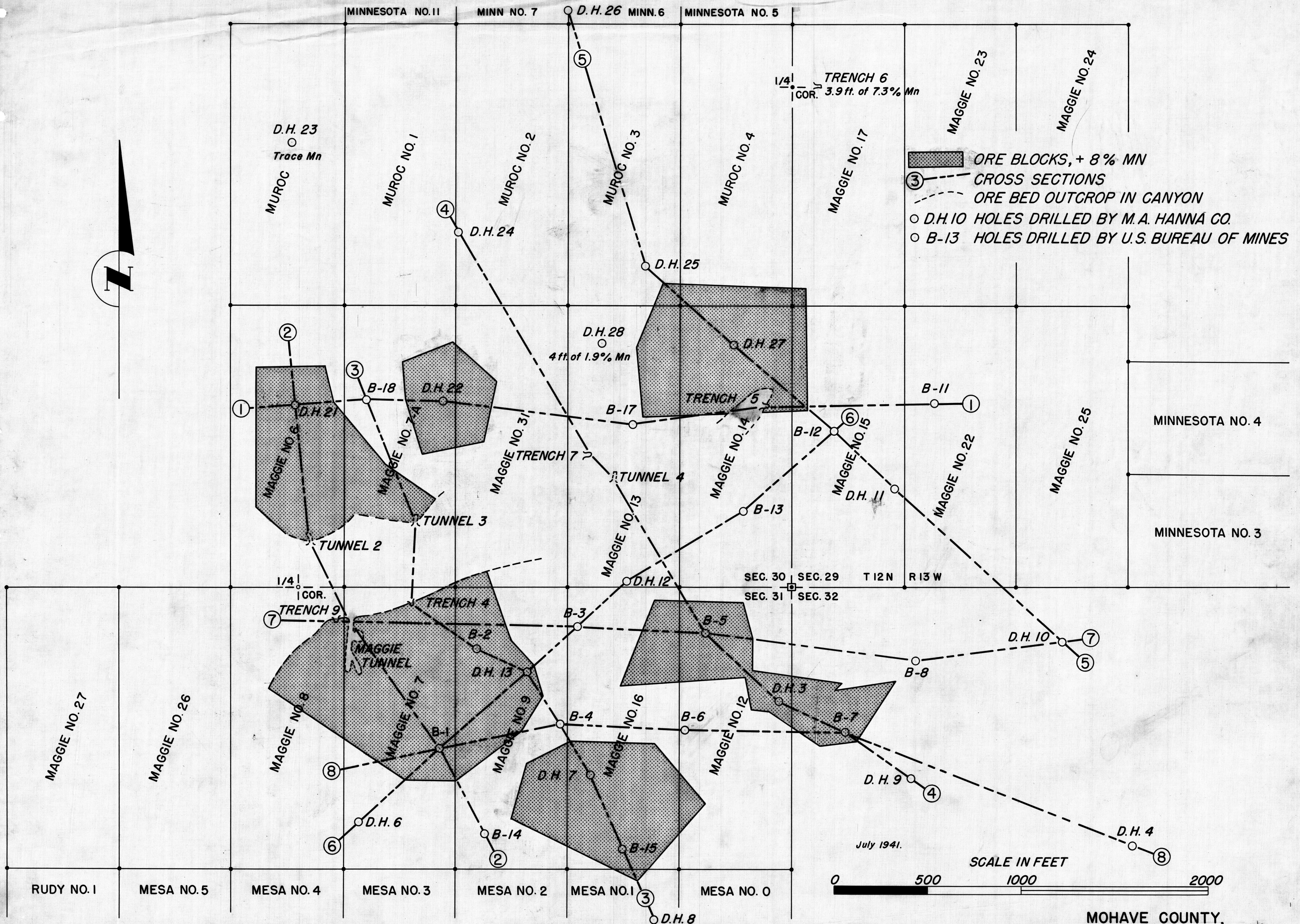
FIG. 5 - ORE BLOCKS INDICATED BY DRILLING. ARTILLERY PEAK MANGANESE DEPOSIT,
