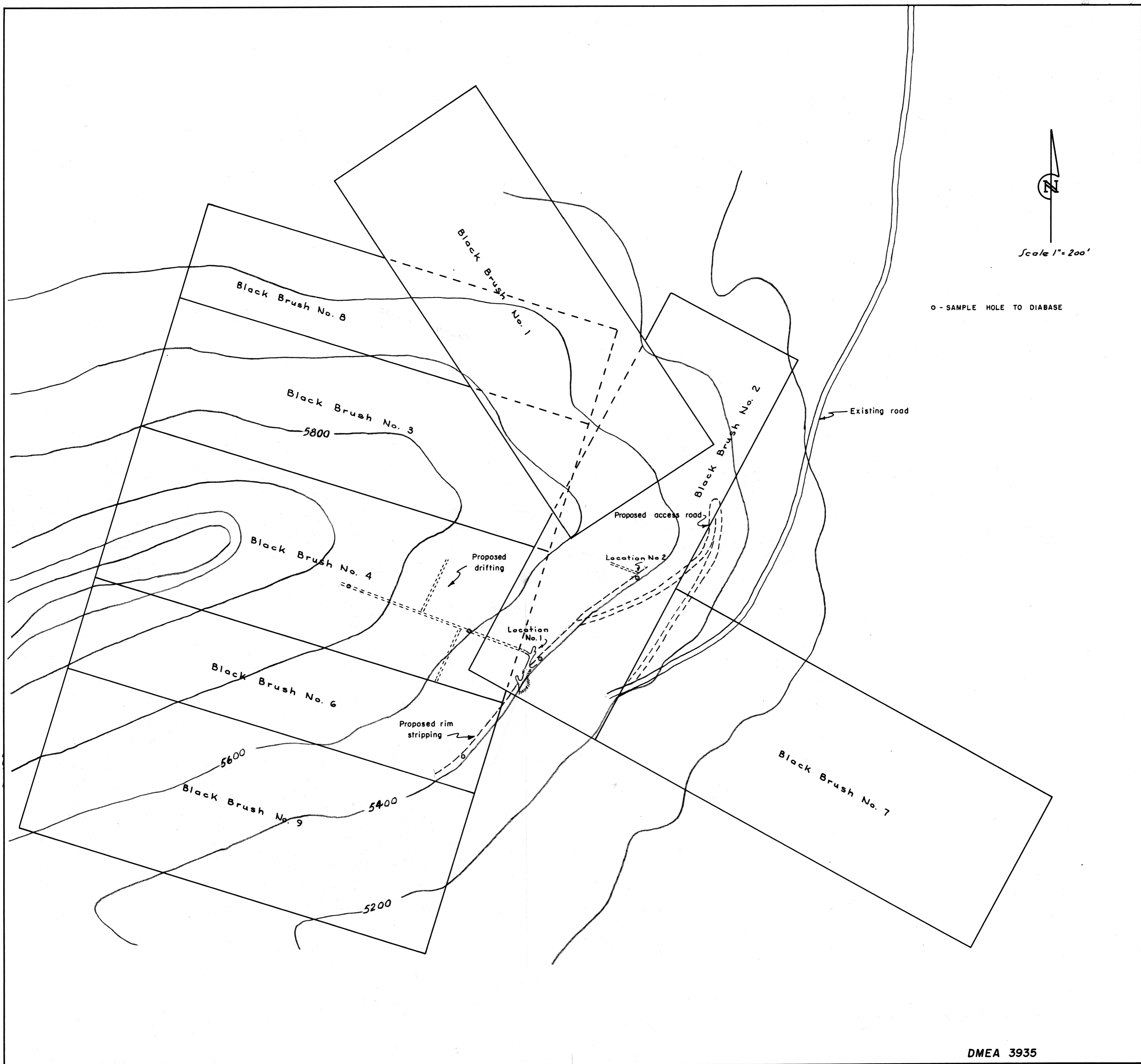
FIG. 4 CLAIM, TOPOGRAPHY, AND PLAN OF PROPOSED PROJECT
