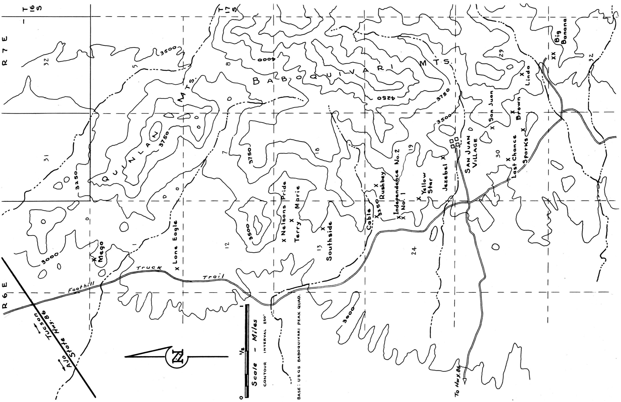
Fig.25-Location Map of Tungsten Deposits, Northern Baboquivari Mountains Area
