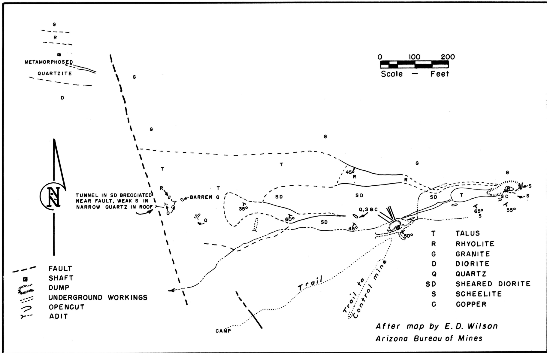
Fig.45-Geologic Map of Taylor X Scheelite deposit, Pima County, Ariz.
