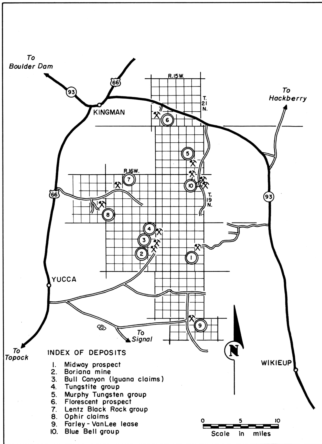
Figure 31. Location map of deposits in the Hualpai mountains, Mohave County, Ariz.
