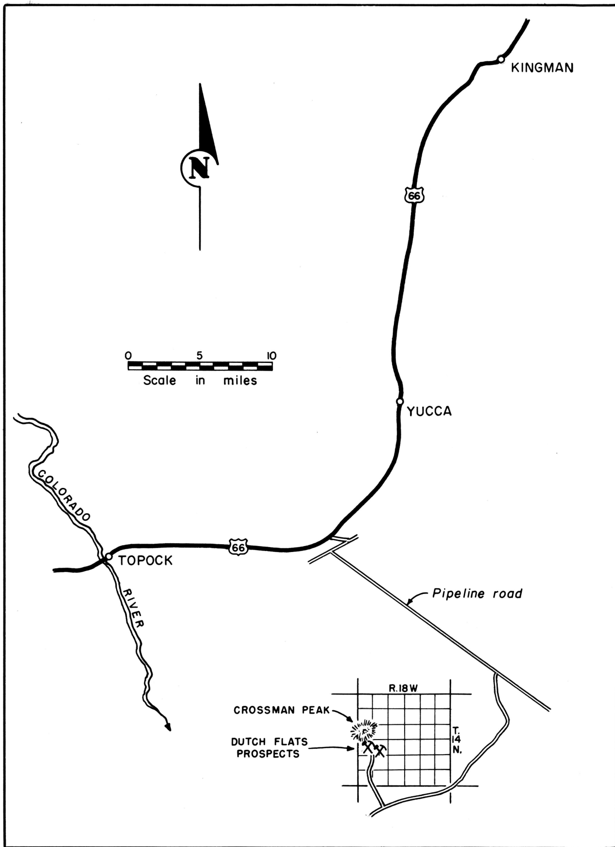
Figure 40.-Location map of Dutch Flats tungsten prospects, Mohave County, Ariz.
