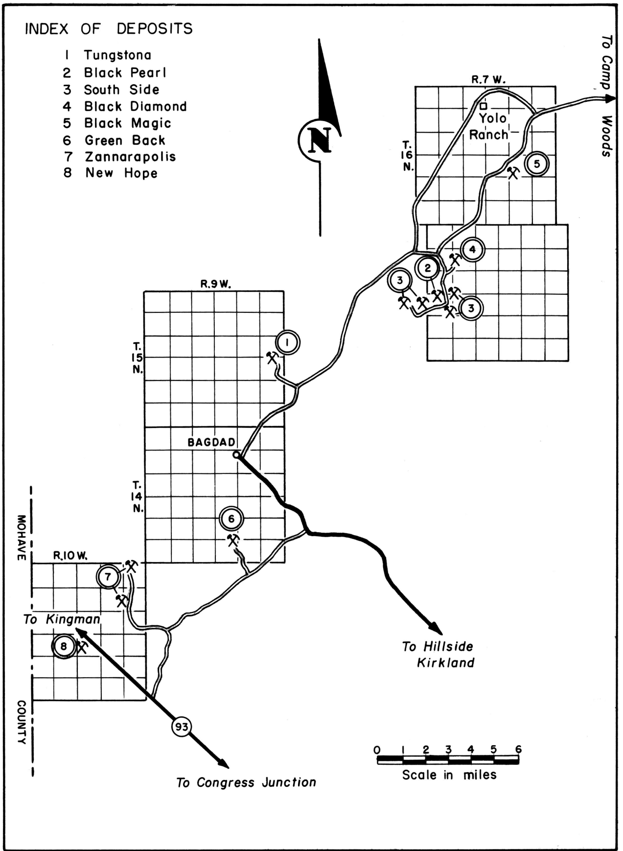
Figure 17. Location map of tungsten deposits in the Bagdad area, Yavapai County, Ariz.
