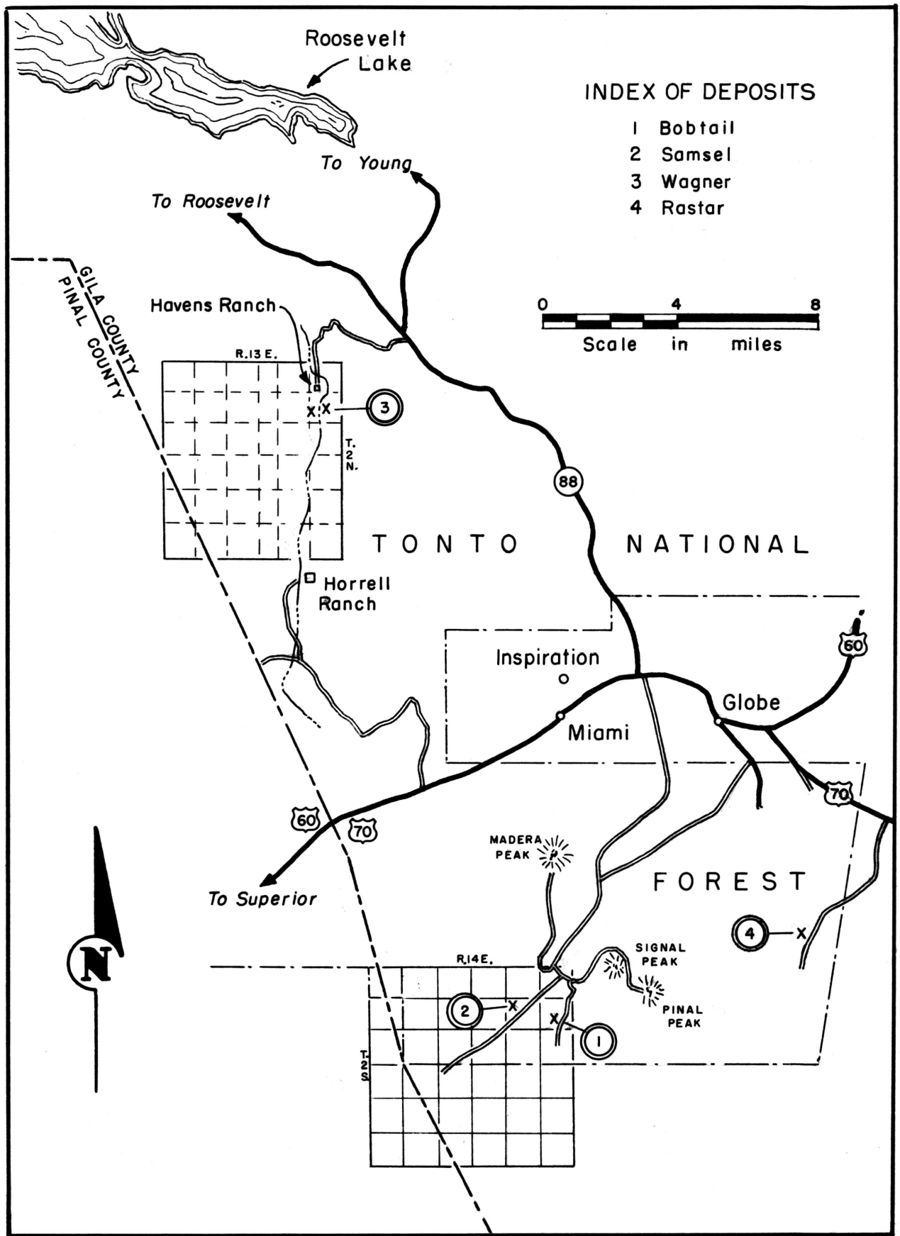
Figure 1 - Location map of deposits in Globe area, Gila County, Ariz.
