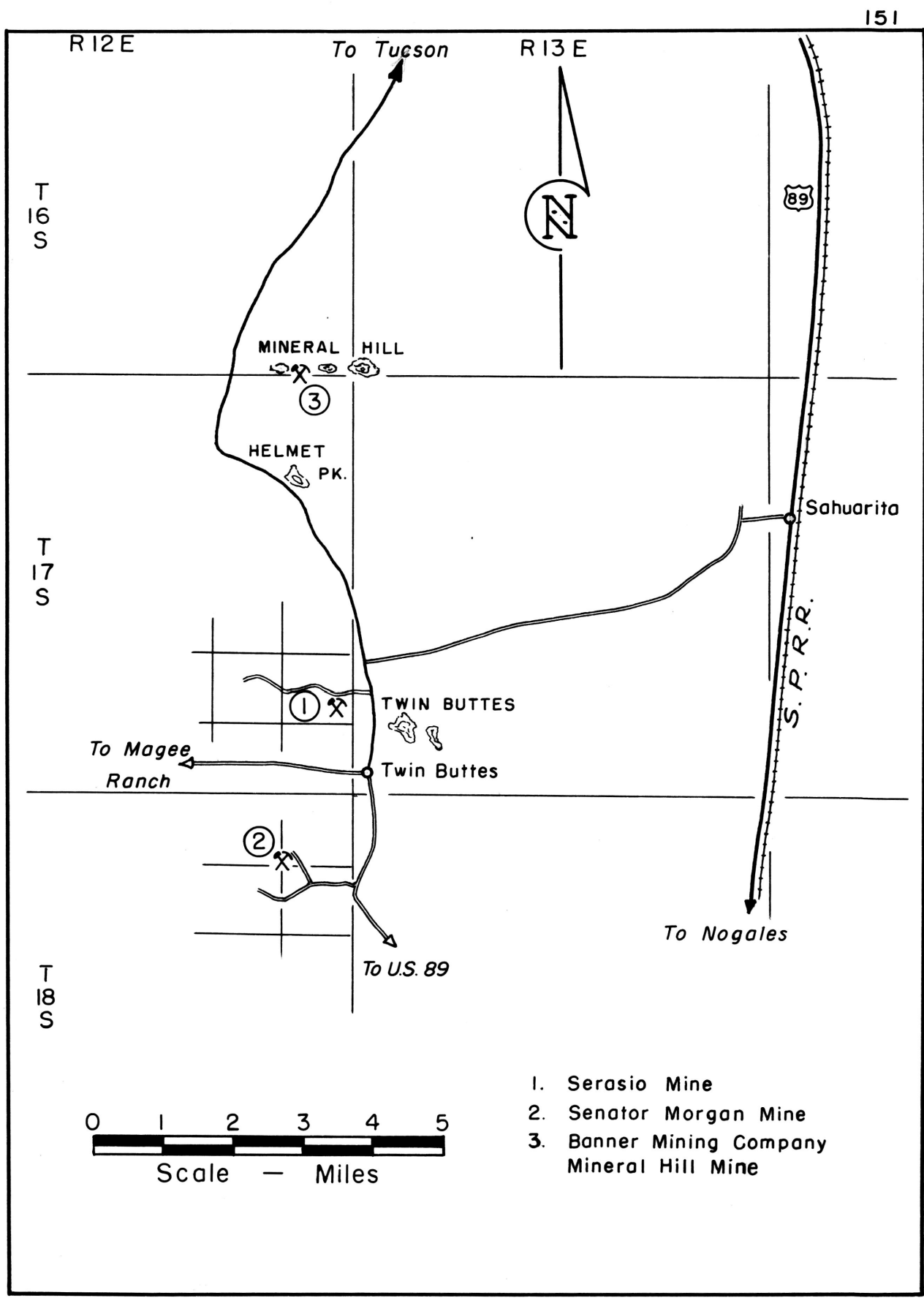
Fig.29-Location Map of Tungsten Deposits in Mineral Hill-Twin Buttes Area, Pima County, Arizona
