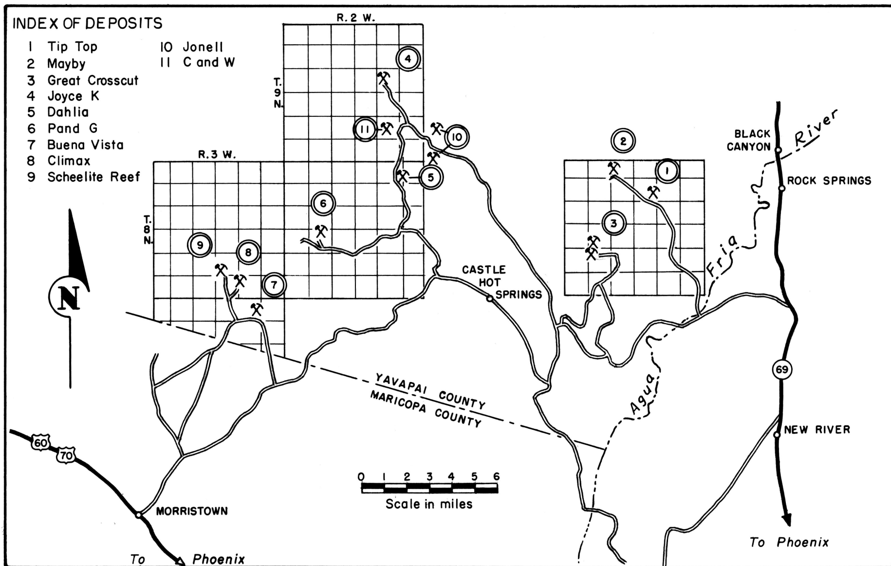
Figure 15. Location map of tungsten deposits in the Tip Top, Castle Creek, and White Picacho districts, Yavapai County, Ariz.
