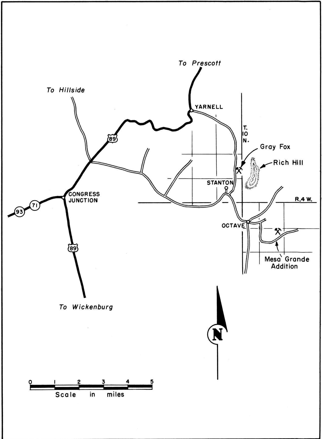
Figure 16. Location map of the Gray Fox and Mesa Grande Addition prospects, Yavapai County, Ariz.
