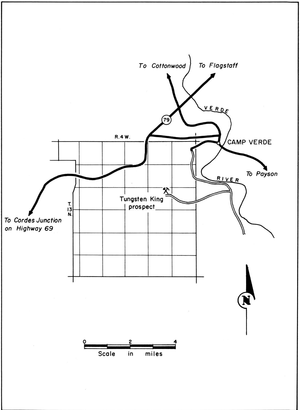
Figure 29. Location map of the Tungsten King prospect, Yavapai County, Ariz.
