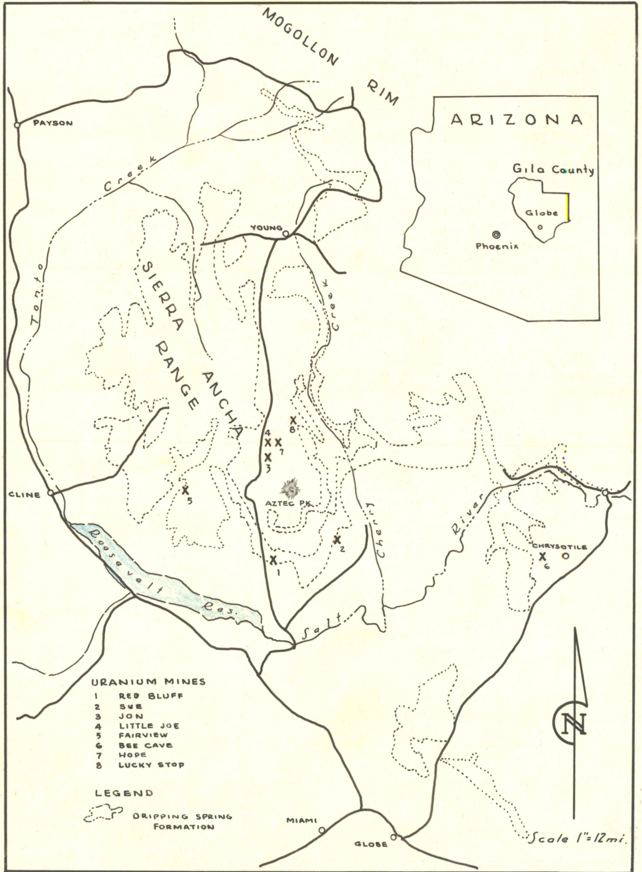
RECONNAISSANCE MAP DRIPPING SPRINGS QUARTZITE FORMATION SIERRA ANCHA DISTRICT, GILA COUNTY ARIZONA
