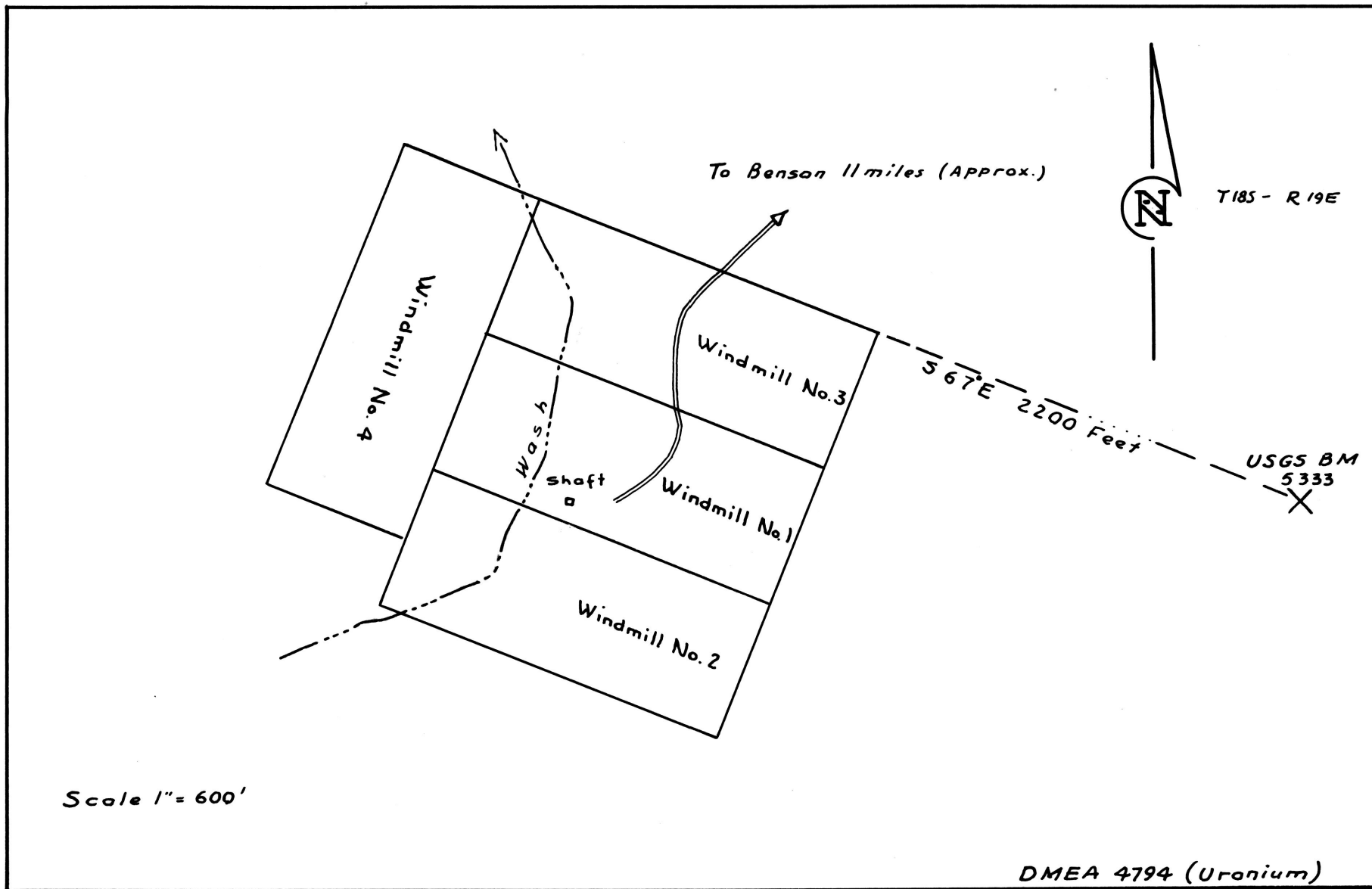
Fig. - 2 - Claim map, Smith-Royston Co. Cochise County, Arizona
