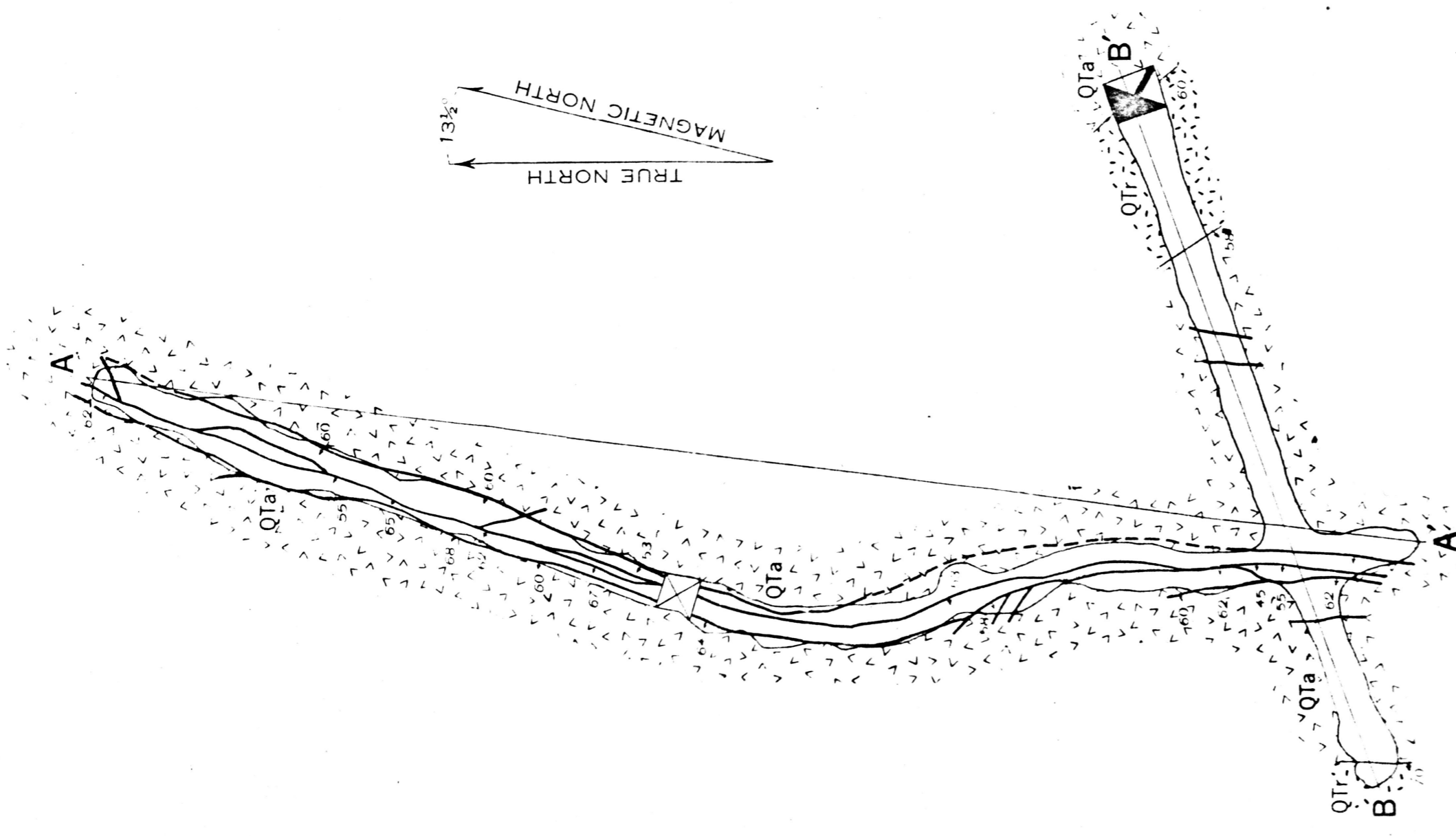
PLAN OF 71-FOOT LEVEL
