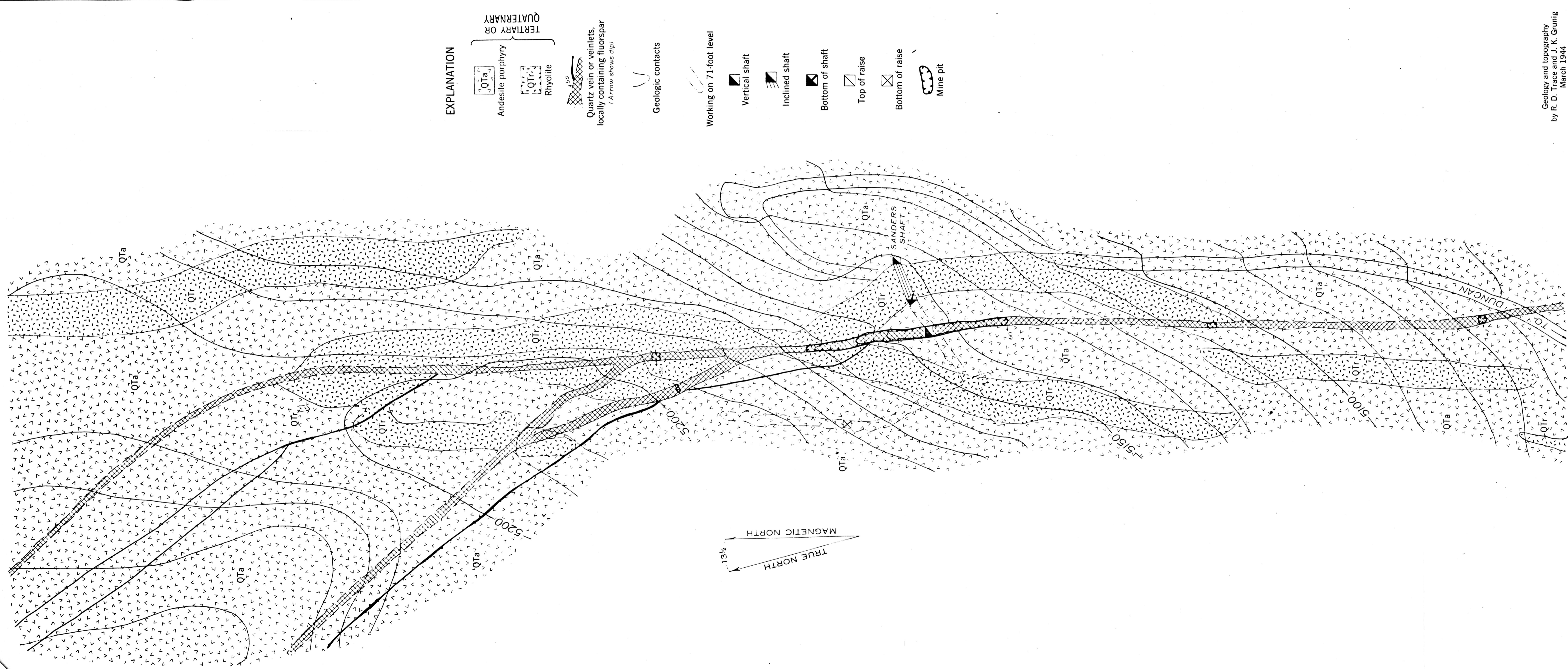
GEOLOGIC AND TOPOGRAPHIC MAP OF THE LUCKIE NO. 1 FLUORSPAR MINE, GREENLEE COUNTY, ARIZONA
