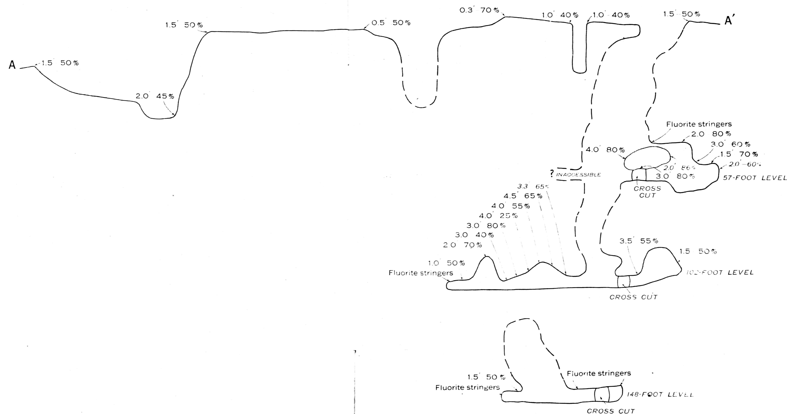
PROJECTION OF THE EAST VEIN ALONG LINE A-A'
