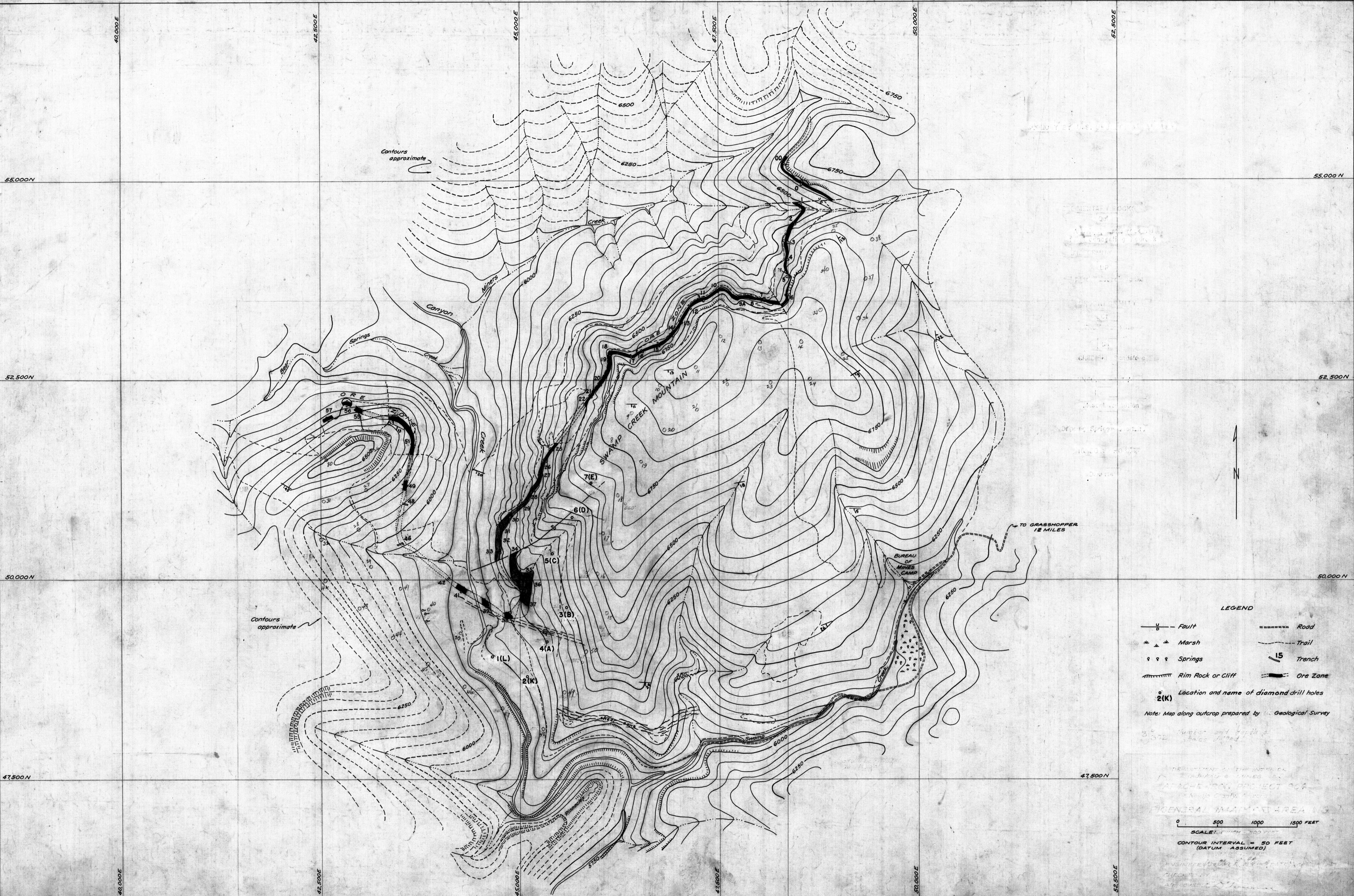
FIG. 3 TOPOGRAPHIC MAP OF APACHE IRON AREA, NAVAJO COUNTY, ARIZONA
