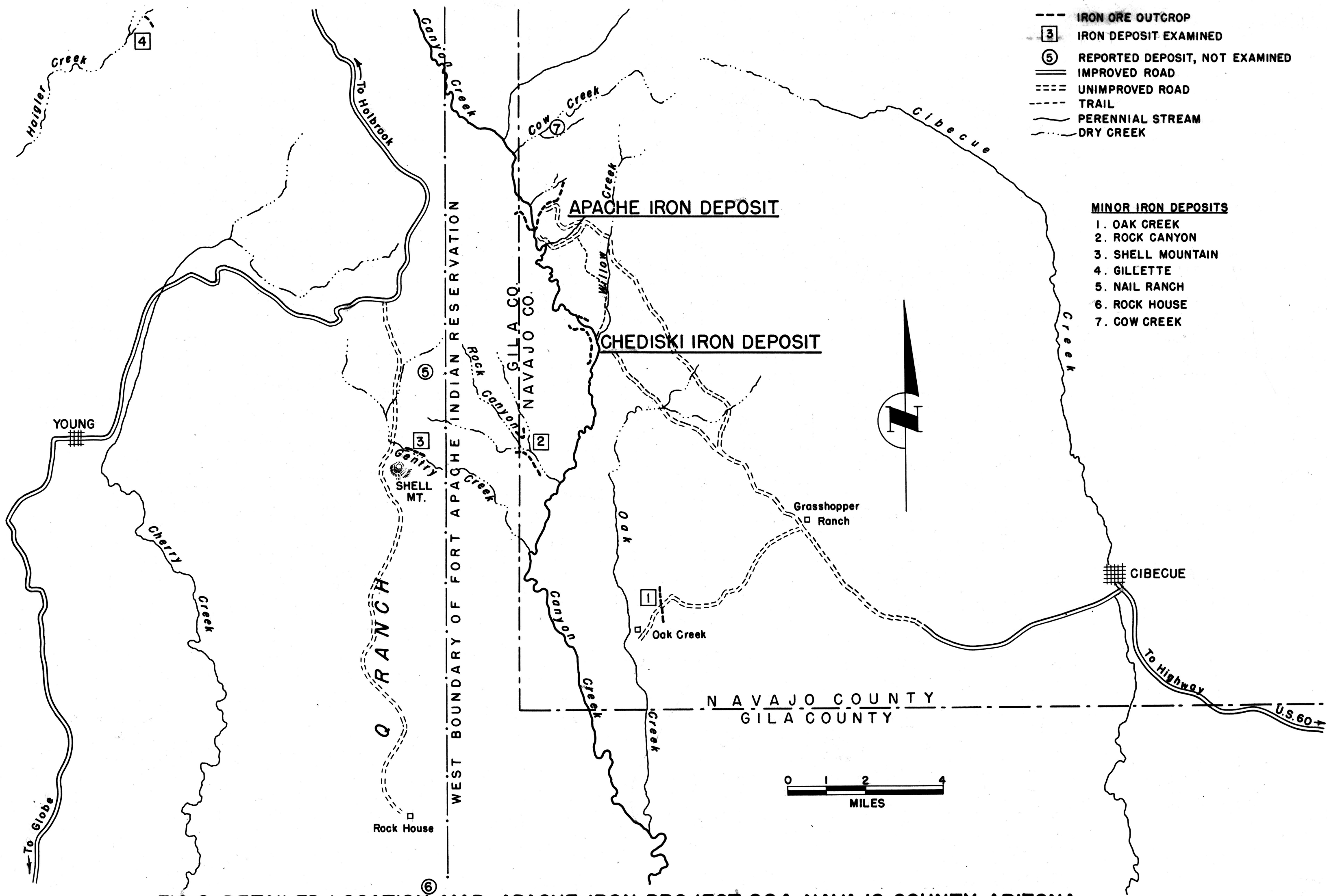
FIG. 2-DETAILED LOCATION MAP, APACHE IRON, PROJECT 904, NAVAJO COUNTY, ARIZONA
