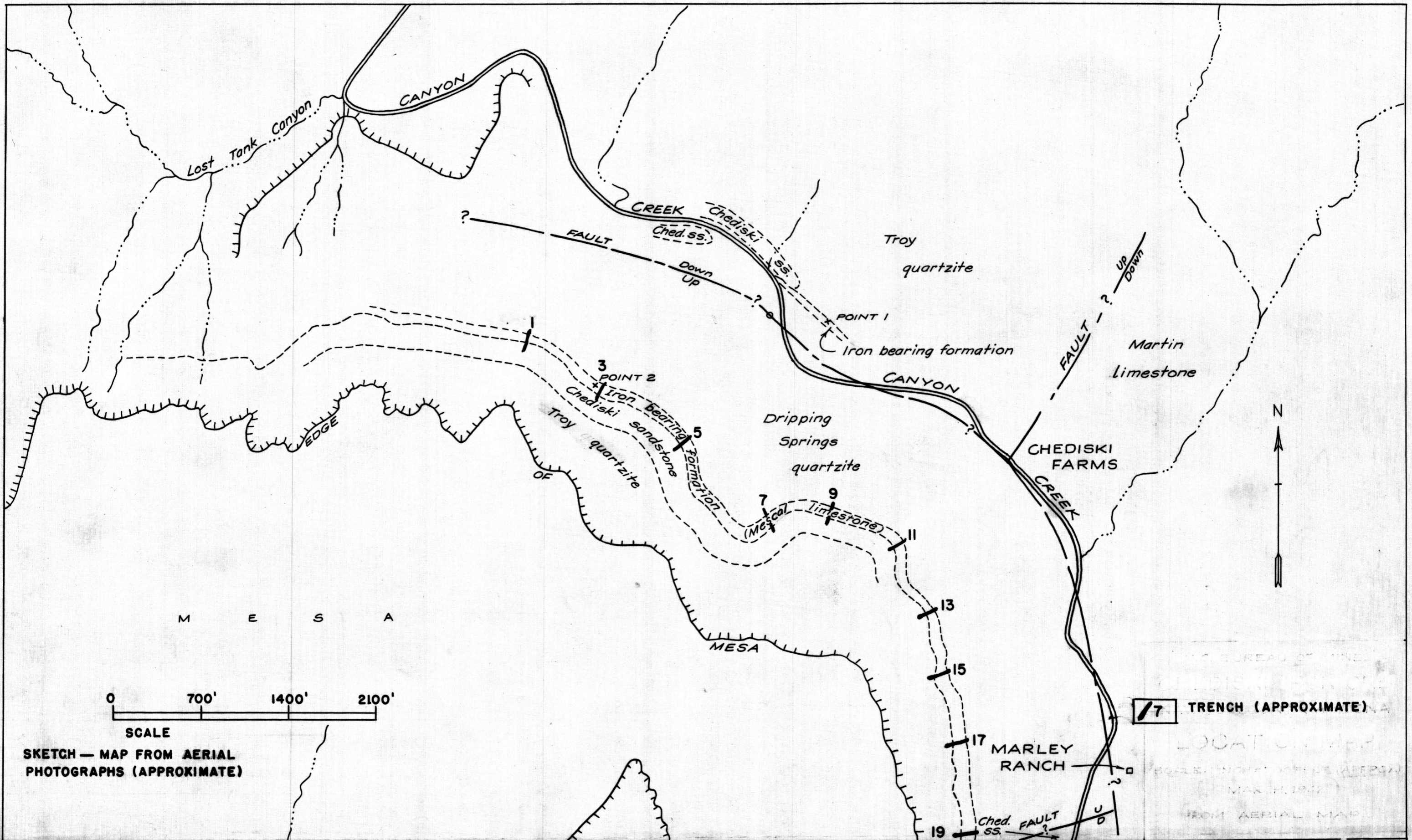
FIG.8 — GEOLOGICAL MAP OF CHEDISKI IRON DEPOSIT — Geology by Geological Survey
