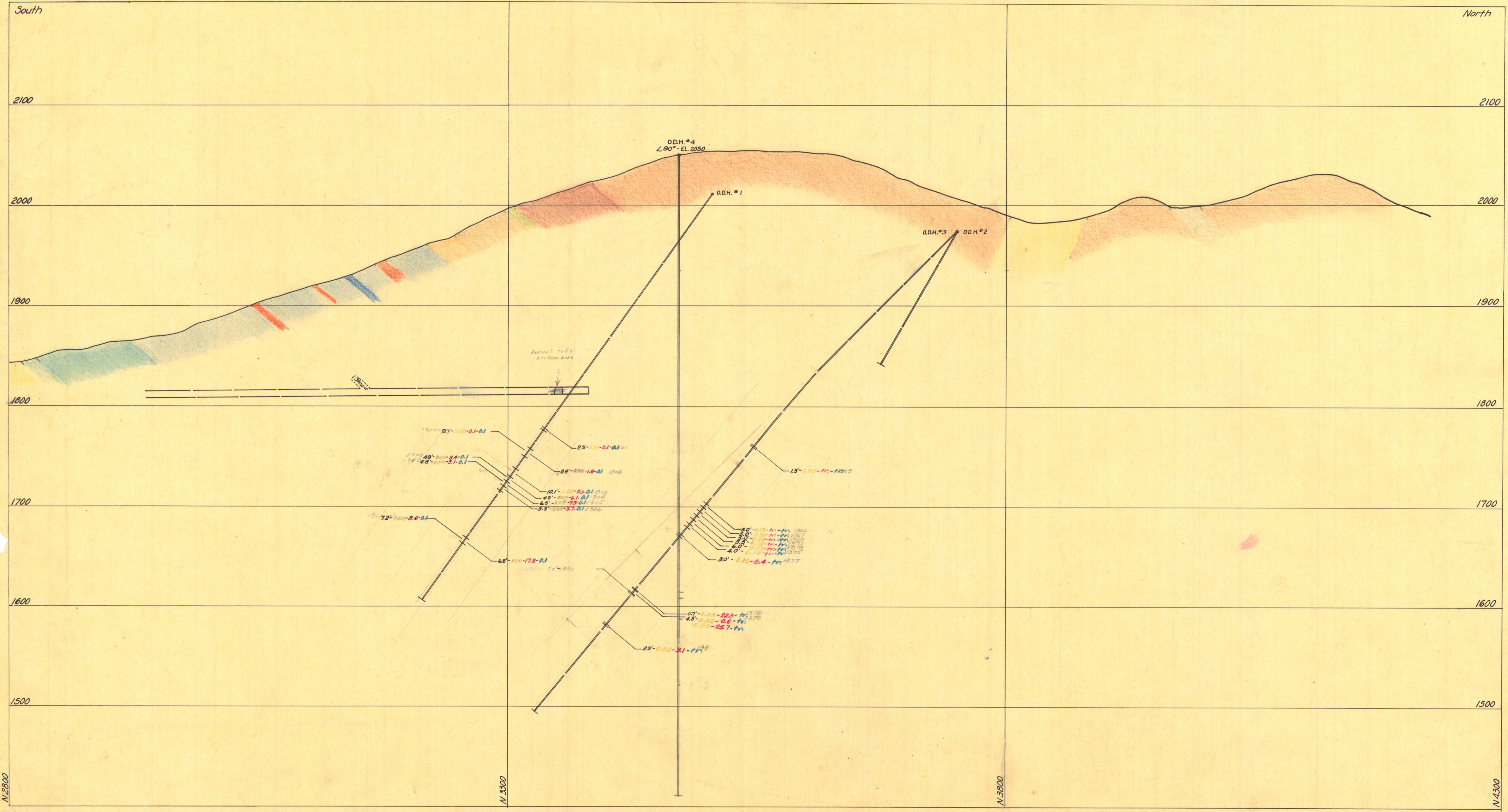
VERTICAL SECTION ON DEPARTURE EAST 9850, LOOKING WEST Scale: 1" = 50'
