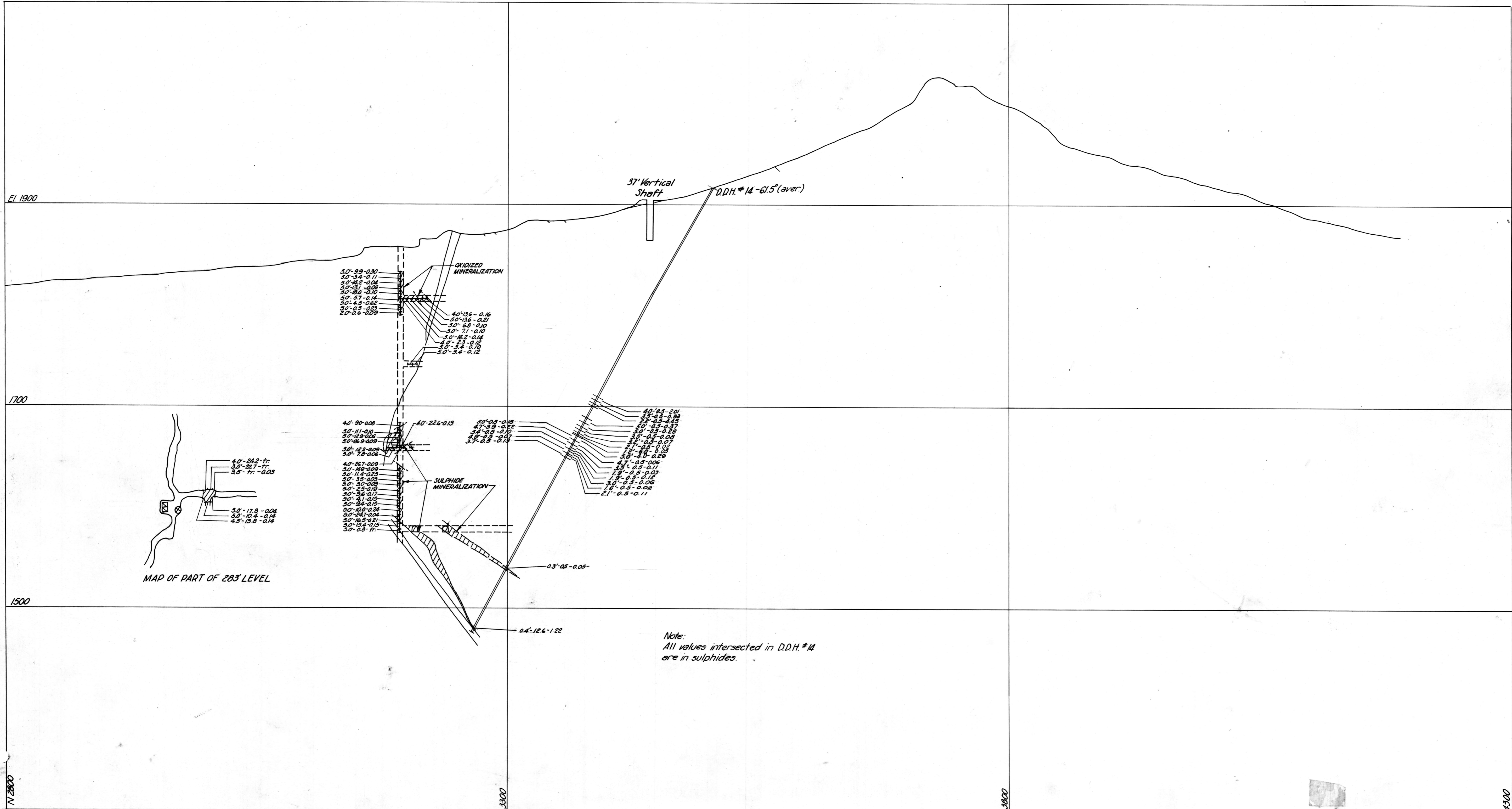
ASSAY SECTION THRU PHONODOREE SHAFT & HOLE NO. 14 Scale: 1"=50'
