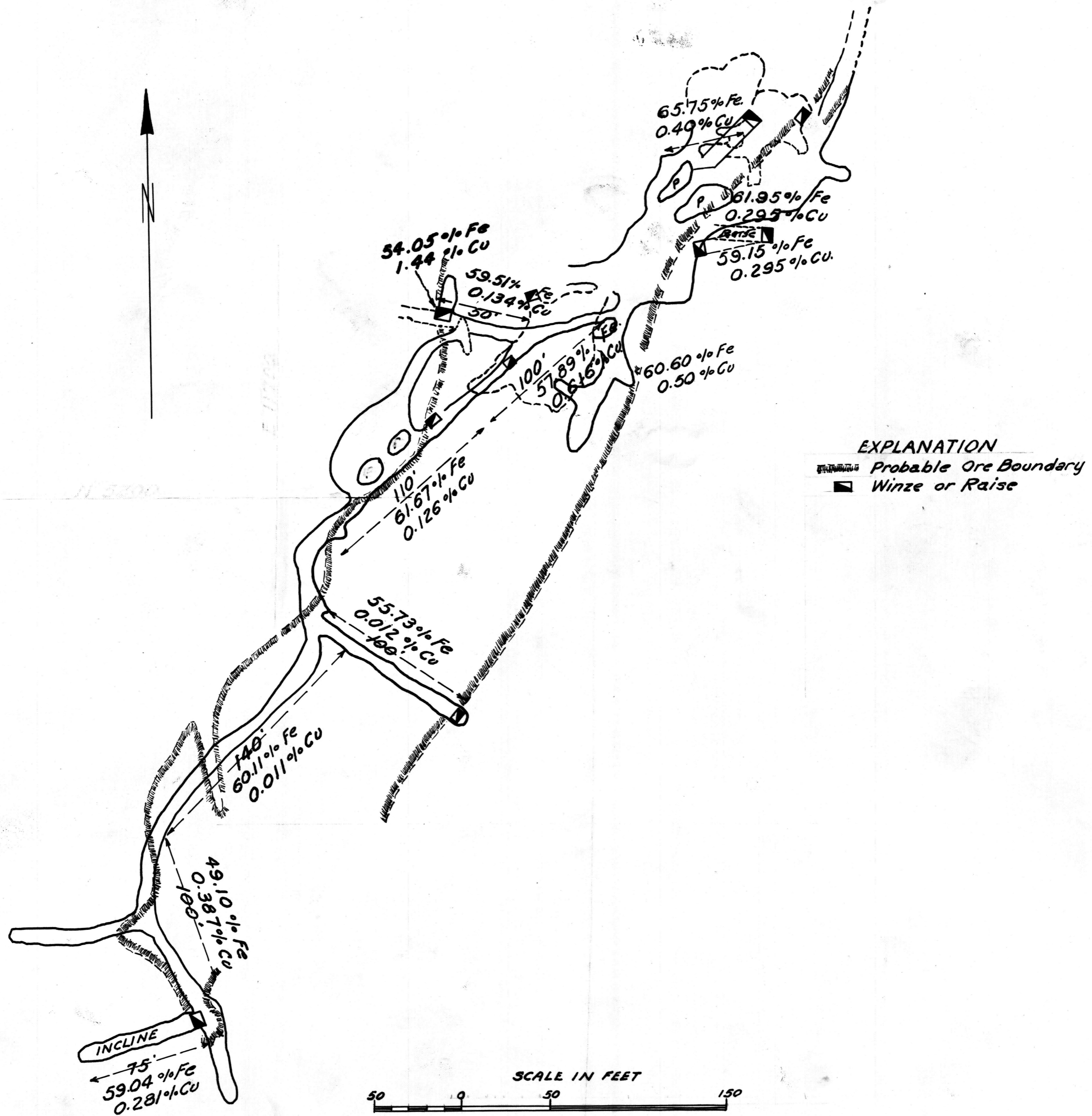
FIG. 4, MAP Showing Average Assays In Part of Incline Workings. NEW PLANET IRON MINE
