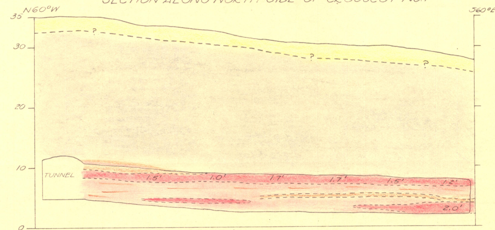
SECTION ALONG SOUTH SIDE OF CROSSCUT No. 2
