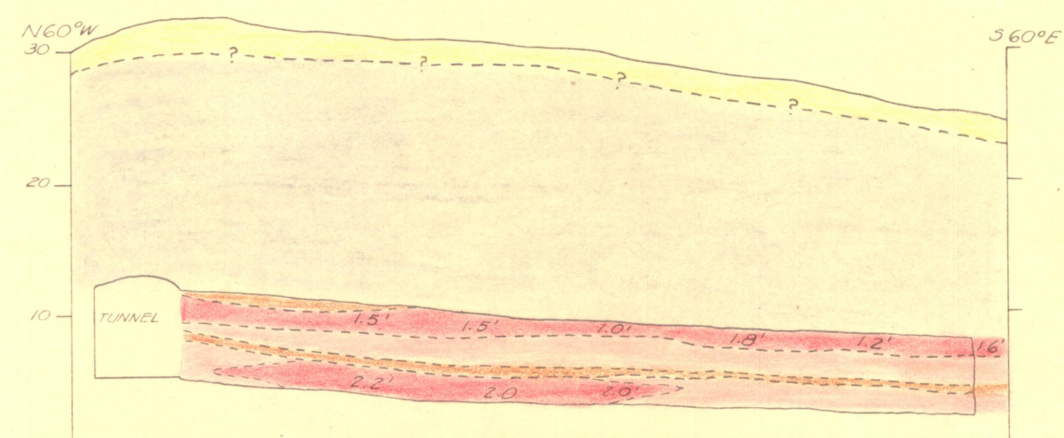
SECTION ALONG NORTH SIDE OF CROSSCUT No. 1
