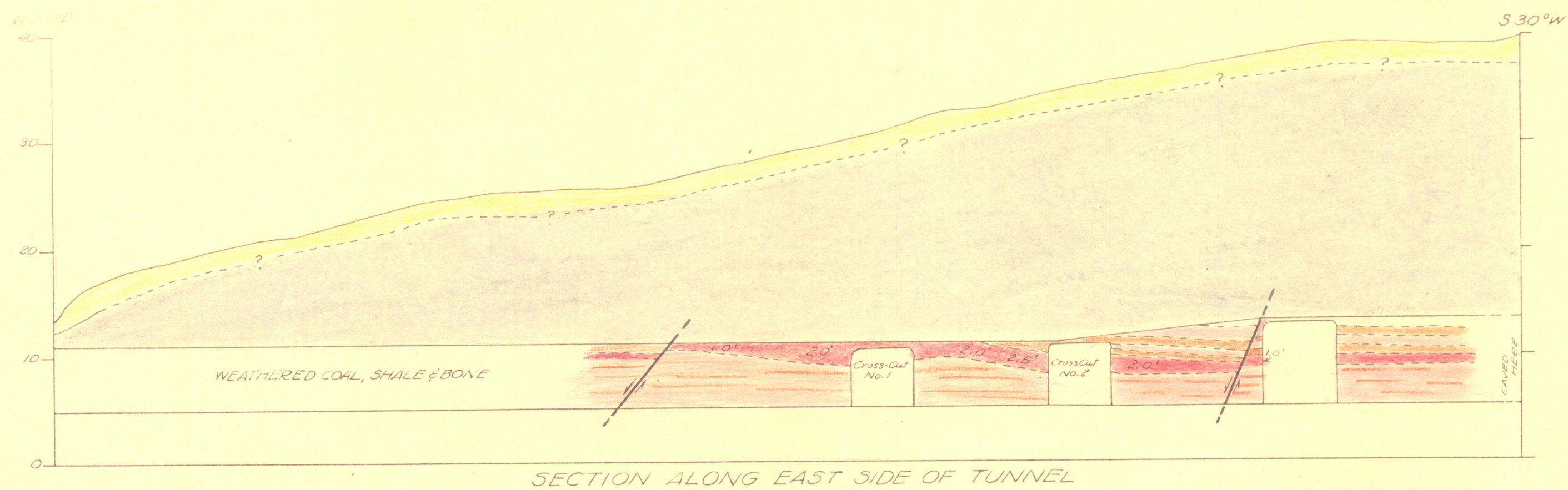
SECTION ALONG EAST SIDE OF TUNNEL
