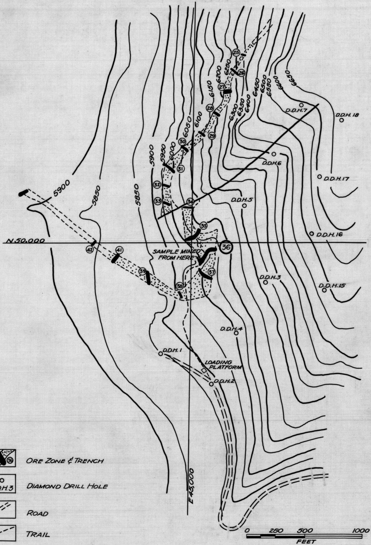
FIG.6-SOUTH END OF APACHE IRON DEPOSIT SHOWING LOCATION OF TRENCH 36
