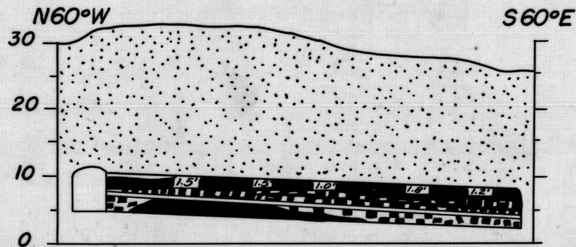
FIG. 4 - SECTION ALONG NORTH SIDE OF CROSSCUT NO. 1
