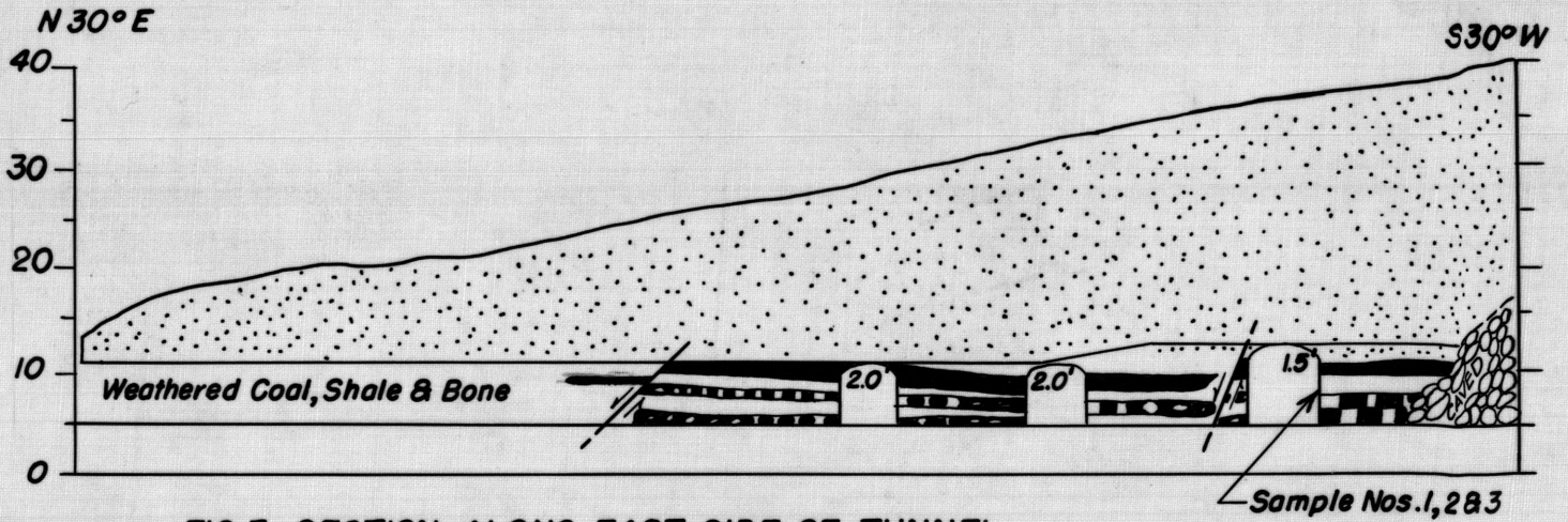
FIG. 3- SECTION ALONG EAST SIDE OF TUNNEL
