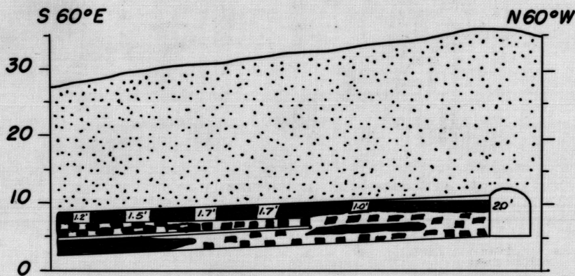
FIG. 5-SECTION ALONG SOUTH SIDE OF CROSSCUT NO. 2
