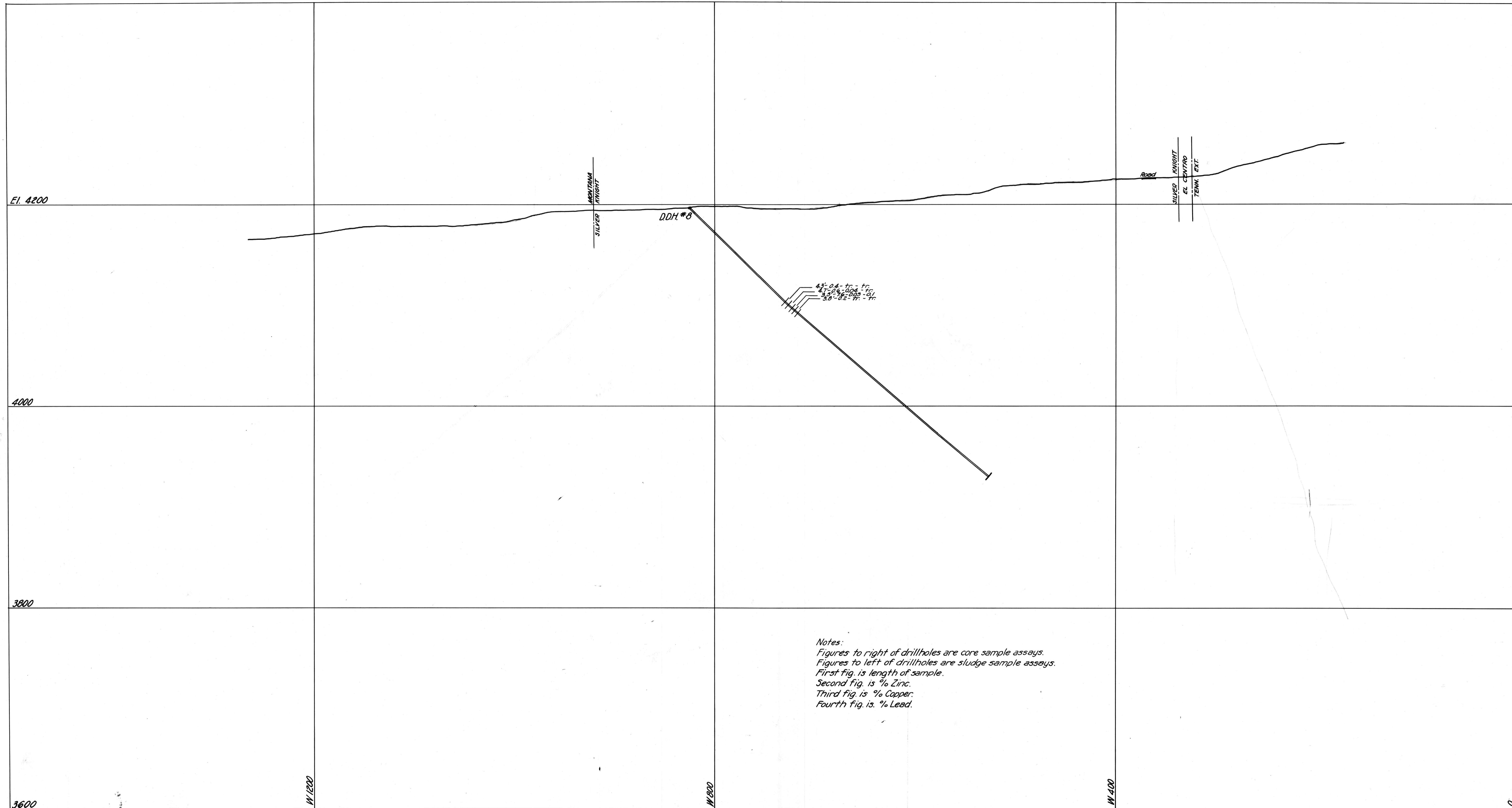
VALUES CUT IN HOLE NO. 8 - JOHNNY BULL & SILVER KNIGHT CLAIMS Scale: 1"=50' Dec. 30, 1943
