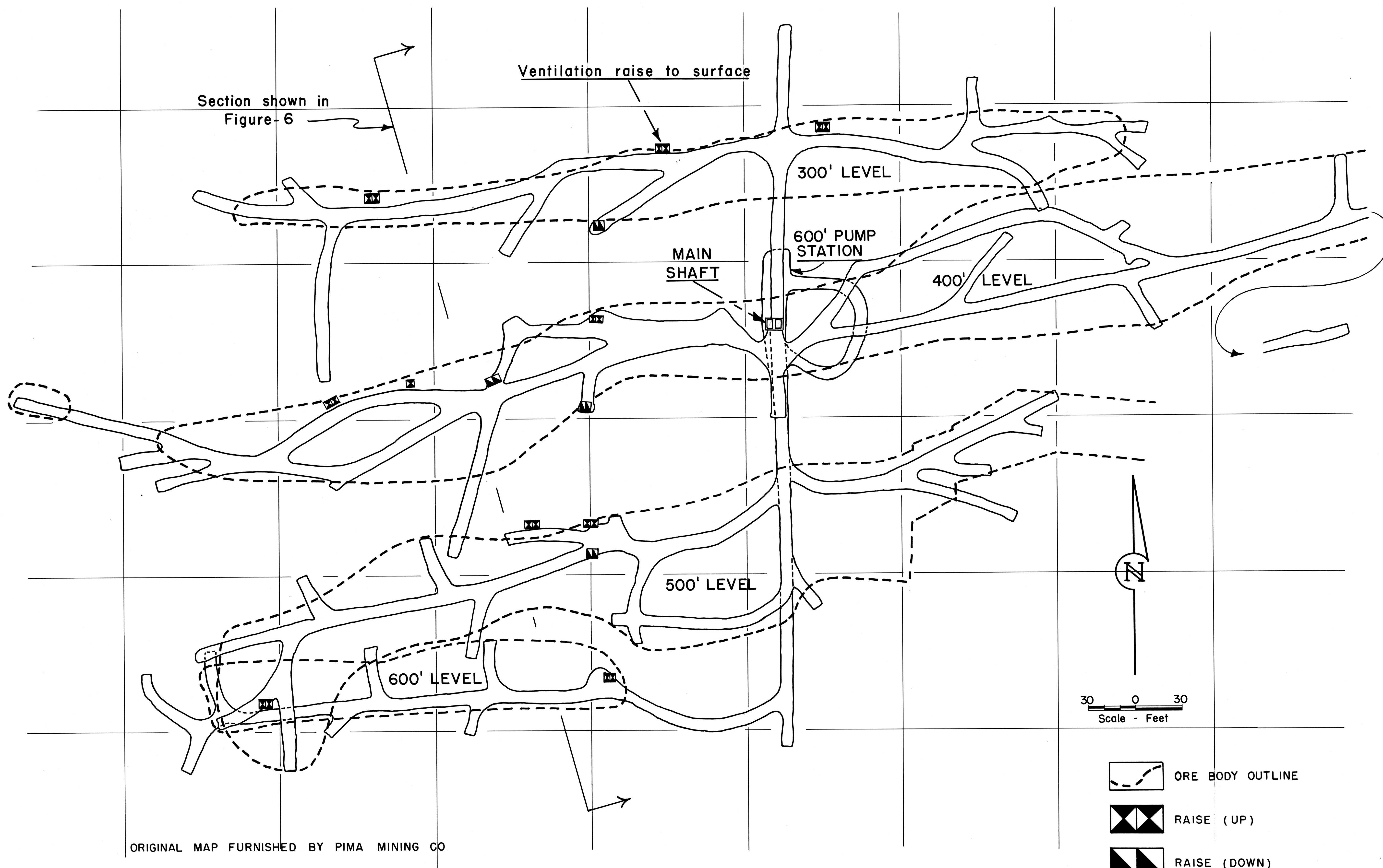
Figure-7- Composite Mine Map
