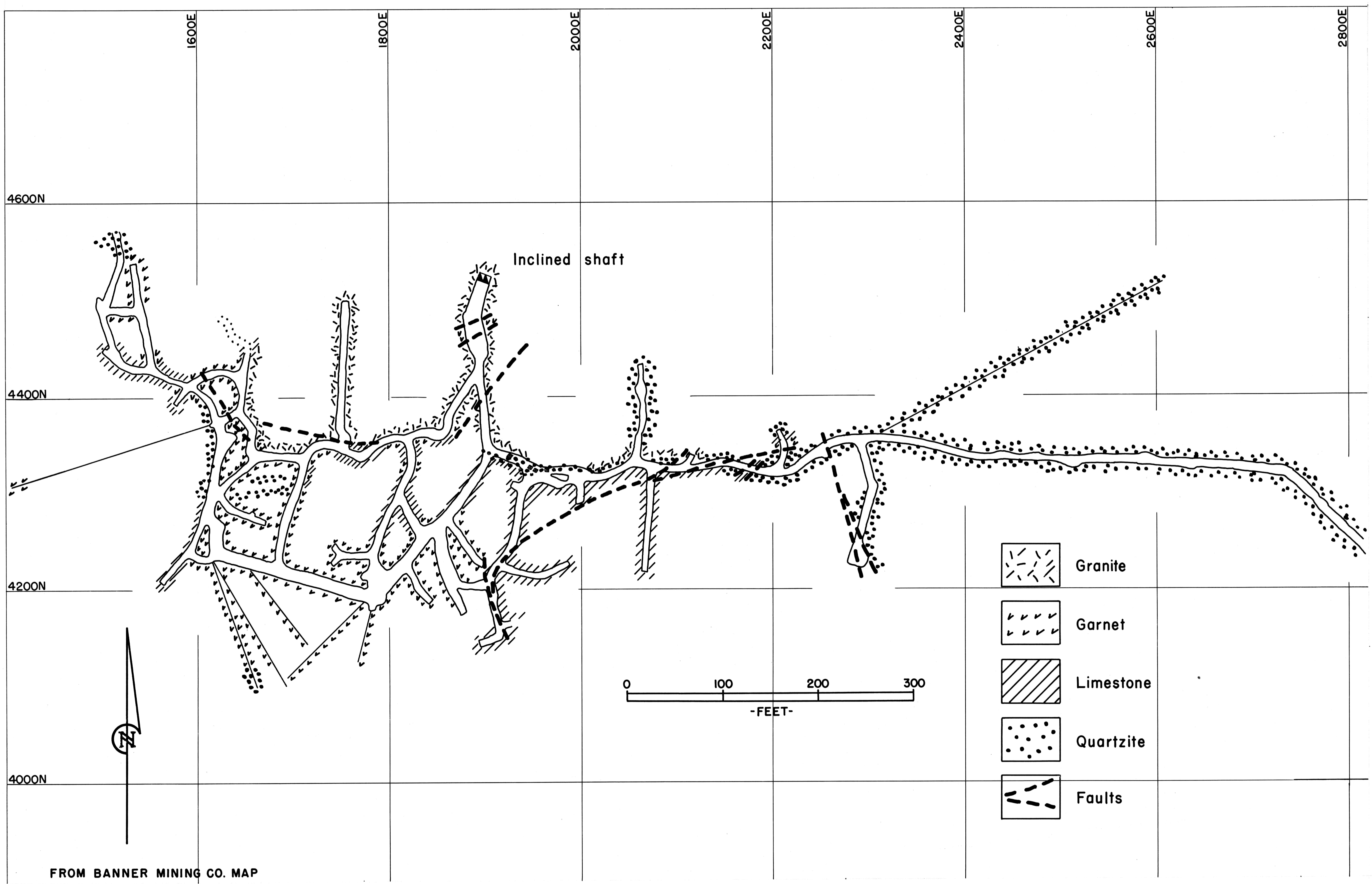
Figure-6- 600 foot level geology.
