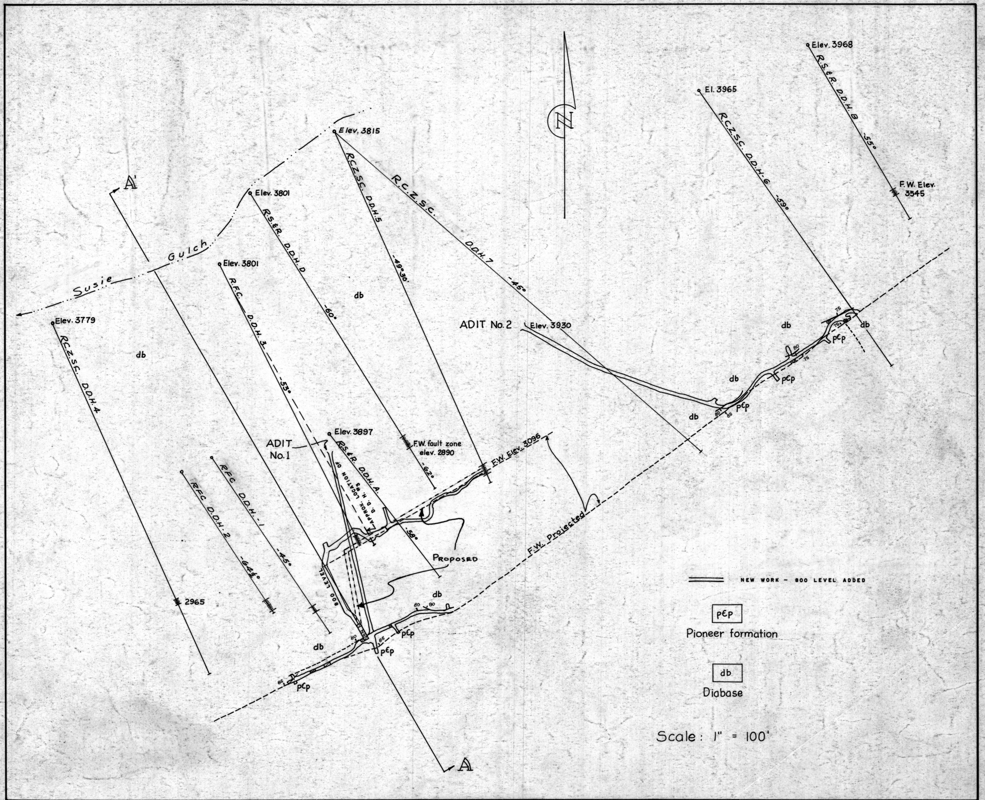
Figure 1, - Plan of Adit No.1 and Adit No.2, POWERFUL Copper Zinc Corporation
