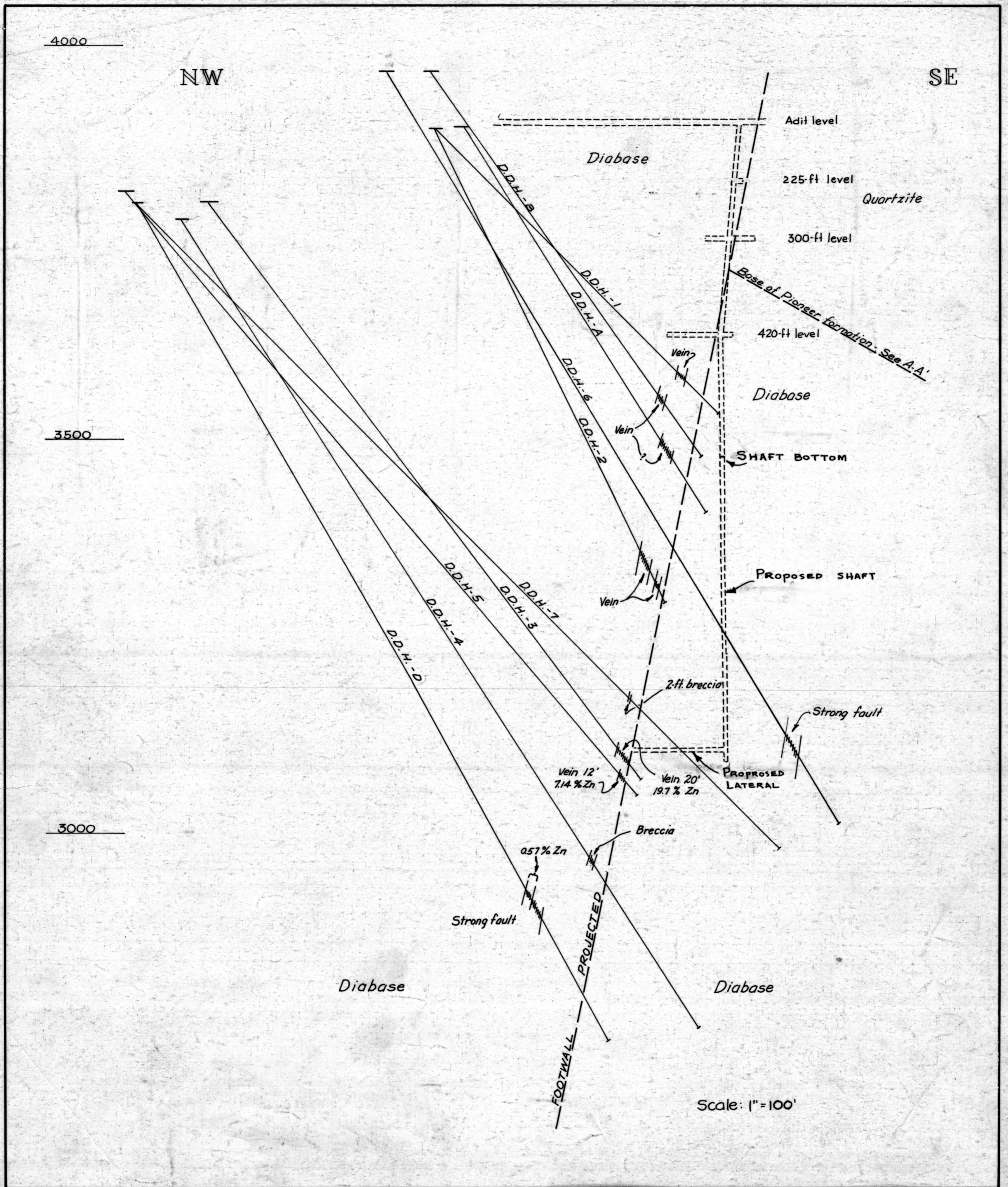
Figure 8, - Composite of drill hole sections, POWERFUL Copper Zinc Corp.
