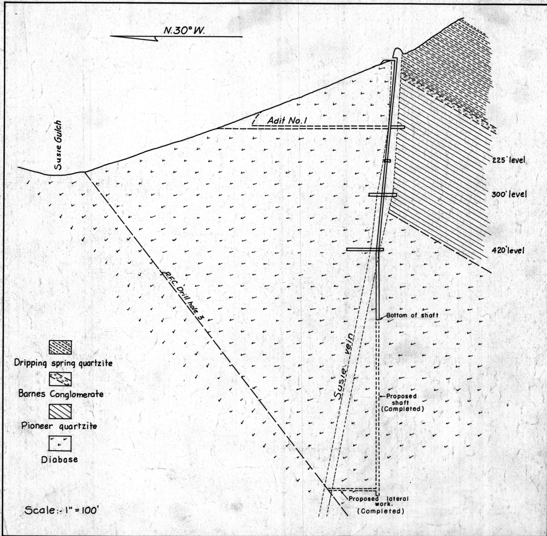
Figure [redacted] - Section A-A' through winze in Adit No. 1, POWERFUL Copper Zinc Corporation
