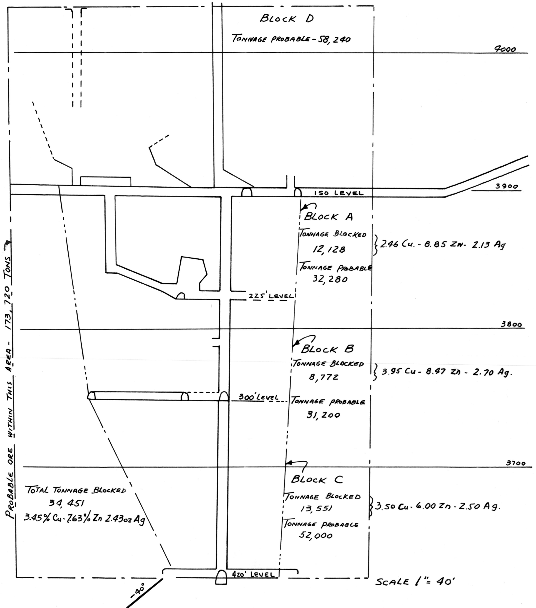
FIGURE 4, - SECTION ON PLANE OF SUSIE VEIN, POWERFUL COPPER-ZINC CORP.
