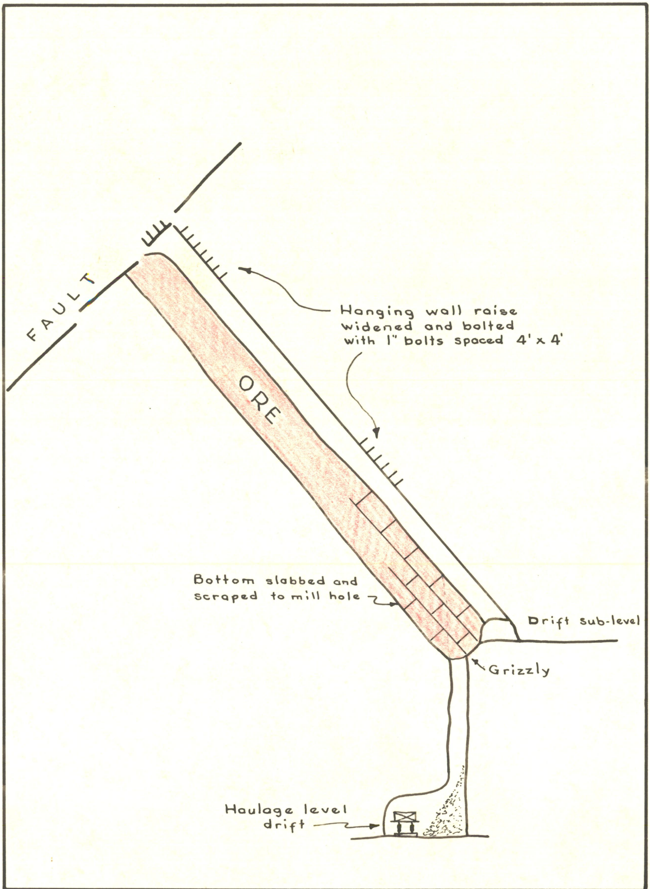
FIG.-3- METHOD OF MINING THIN ORE BODY CORONADO COPPER AND ZINC CO. COCHISE COUNTY, ARIZONA
