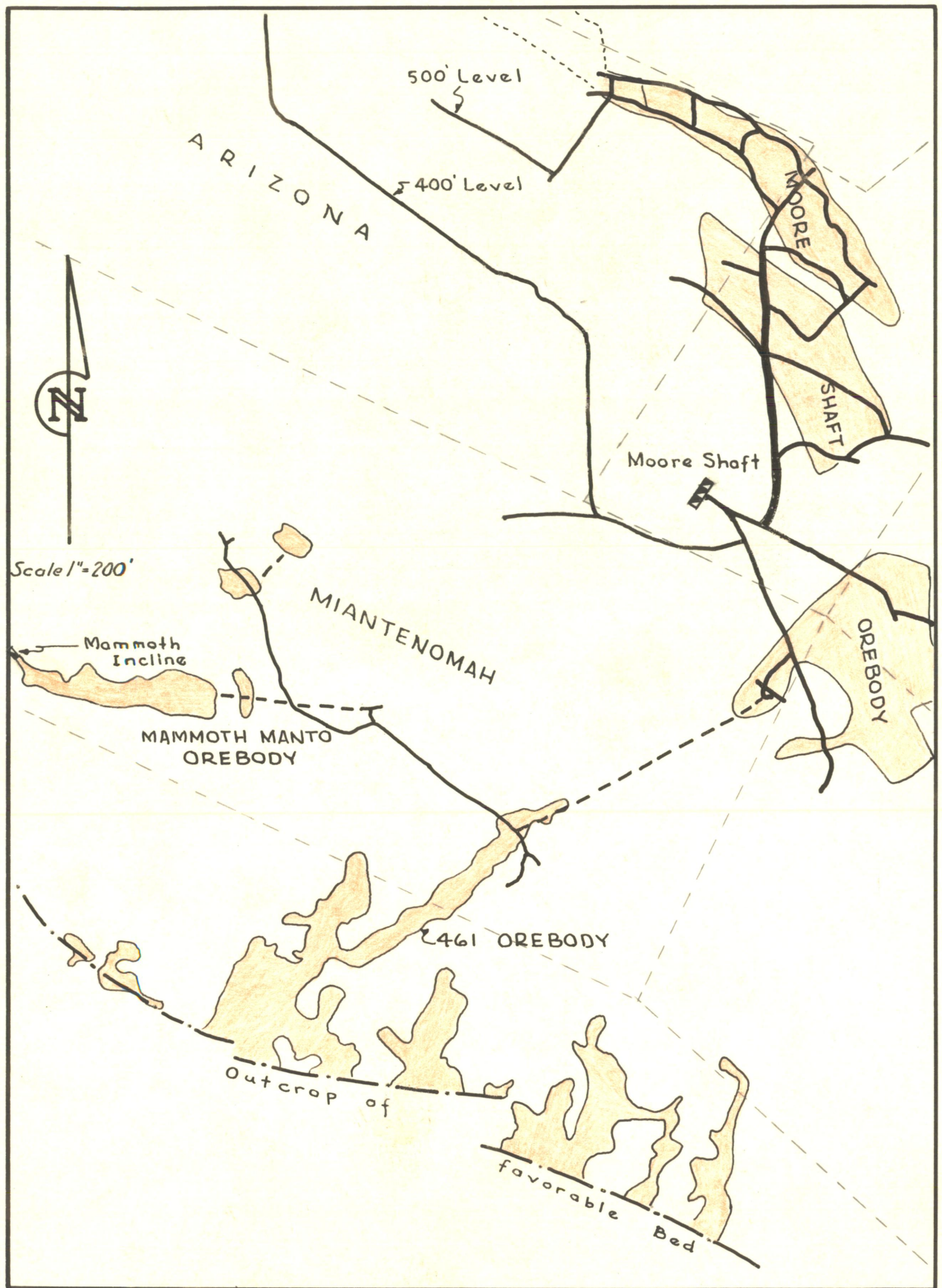
FIG. 2 · MOORE SHAFT ORE BODY CORONADO COPPER & ZINC COMPANY COCHISE COUNTY, ARIZONA
