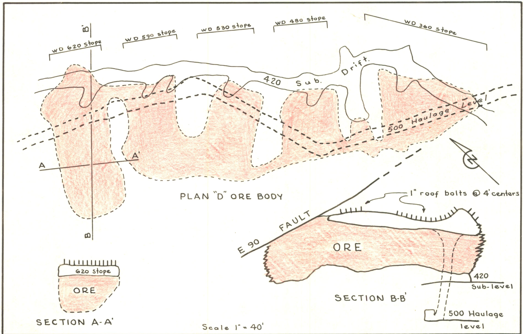
FIG. - 5 - "D" ORE BODY CORONADO COPPER AND ZINC CO. COCHISE COUNTY, ARIZONA
