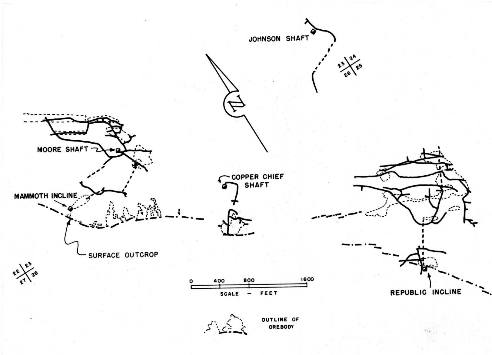
FIGURE -6 - JOHNSON CAMP UNIT, UNDERGROUND WORKINGS
