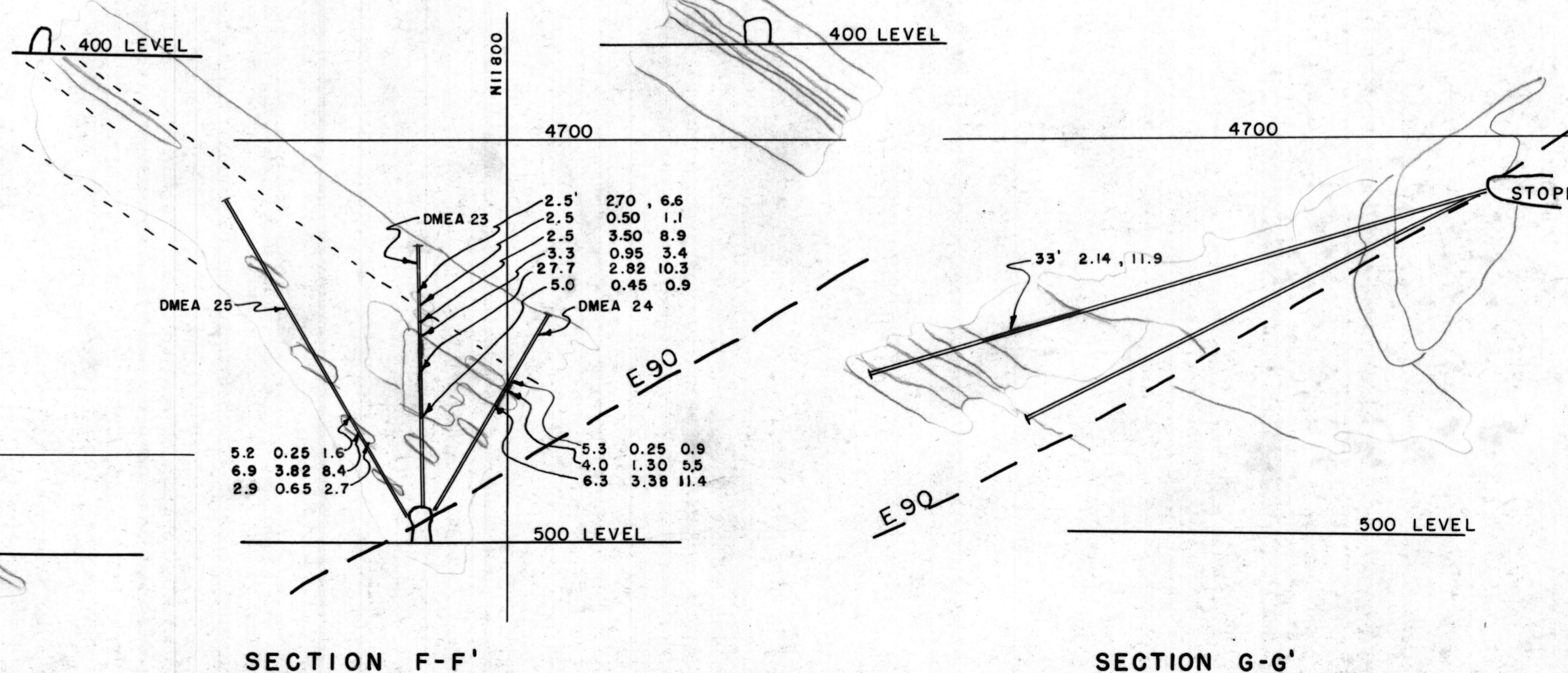
FIG. 4 CORONADO COPPER & ZINC CO. JOHNSON CAMP, ARIZONA AREA I MAP, DMEA DOCKET NO. 2746 SECTIONS THROUGH ORE BODIES DMEA 2746
