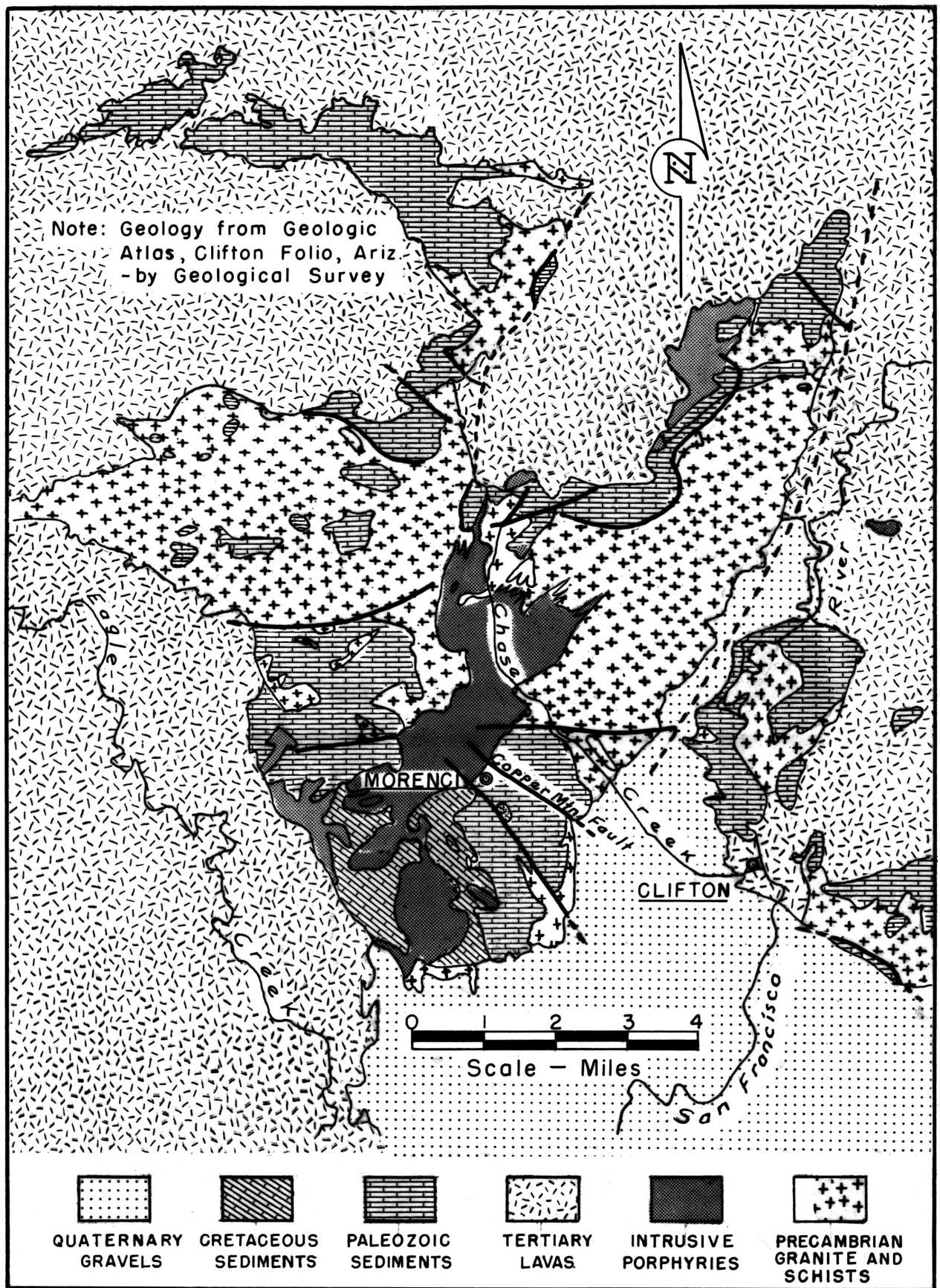
Fig. 5- Generalized Geologic Map of Morenci Area showing the major faults.
